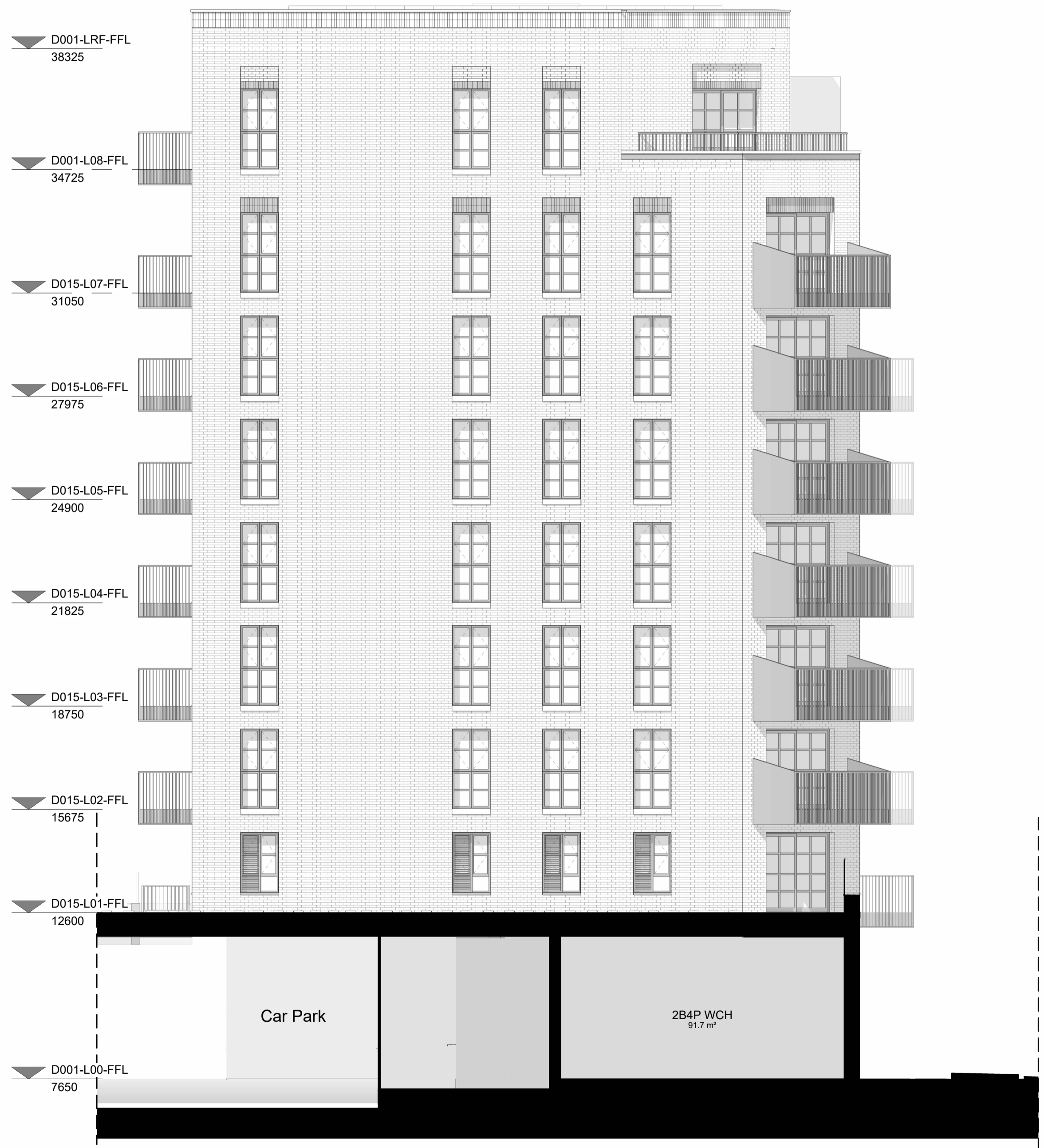
Proposed Block D1 South West Elevation 1 : 100
