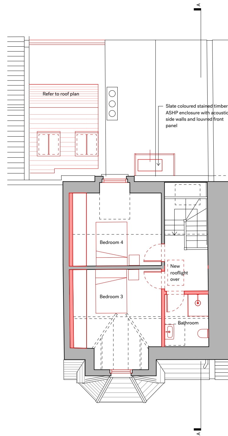
Second Floor
