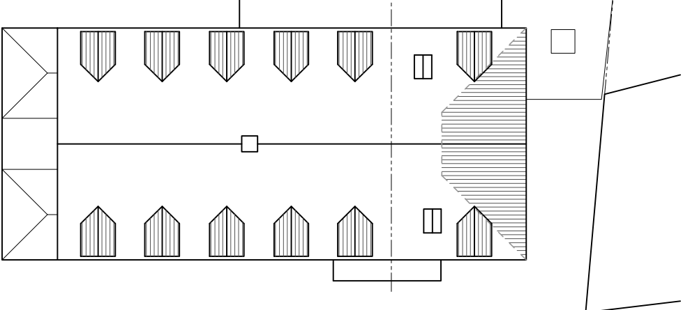
Roof Plan @ 1:100
