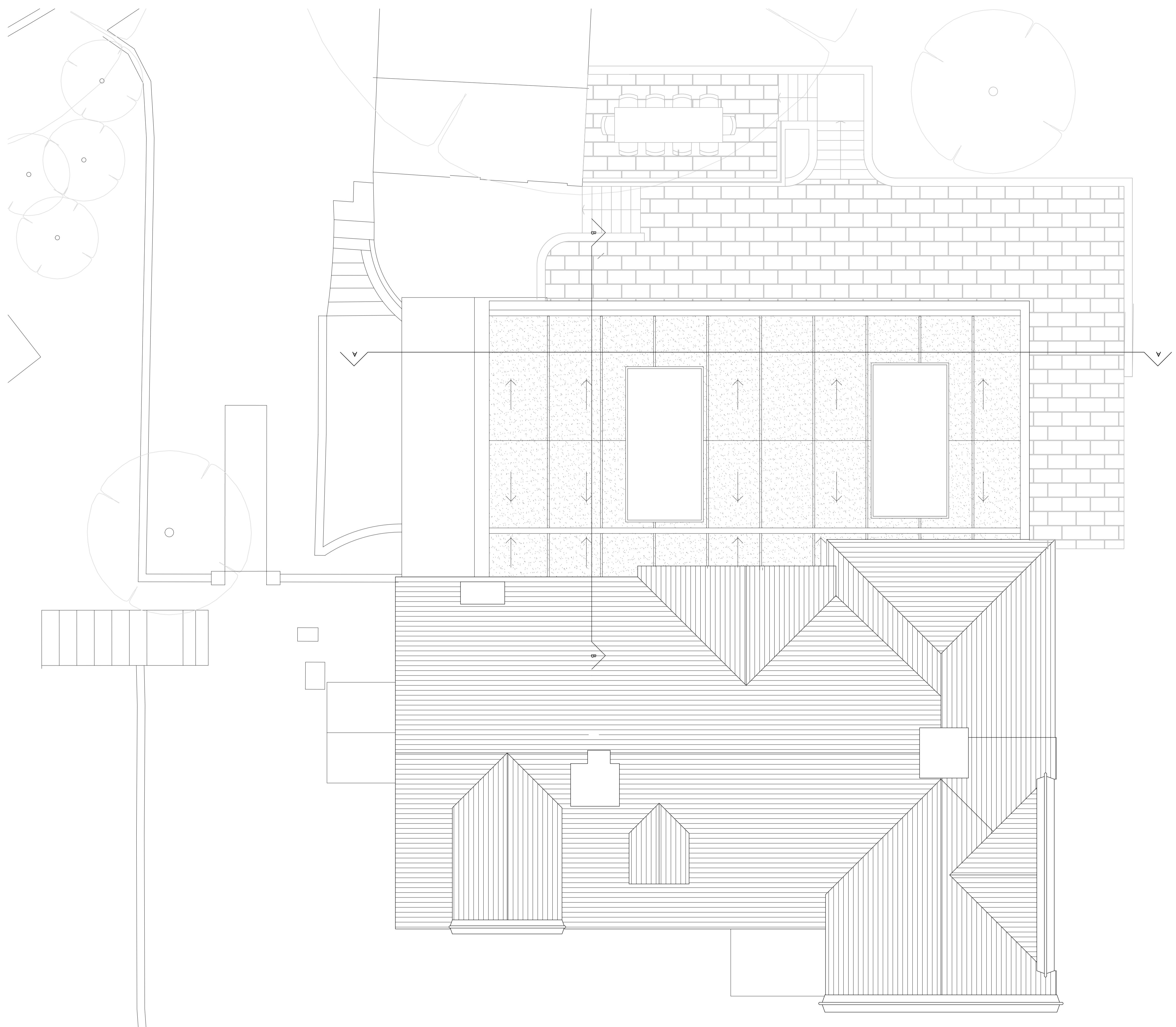
PROPOSED ROOF PLAN Scale 1/ 50
