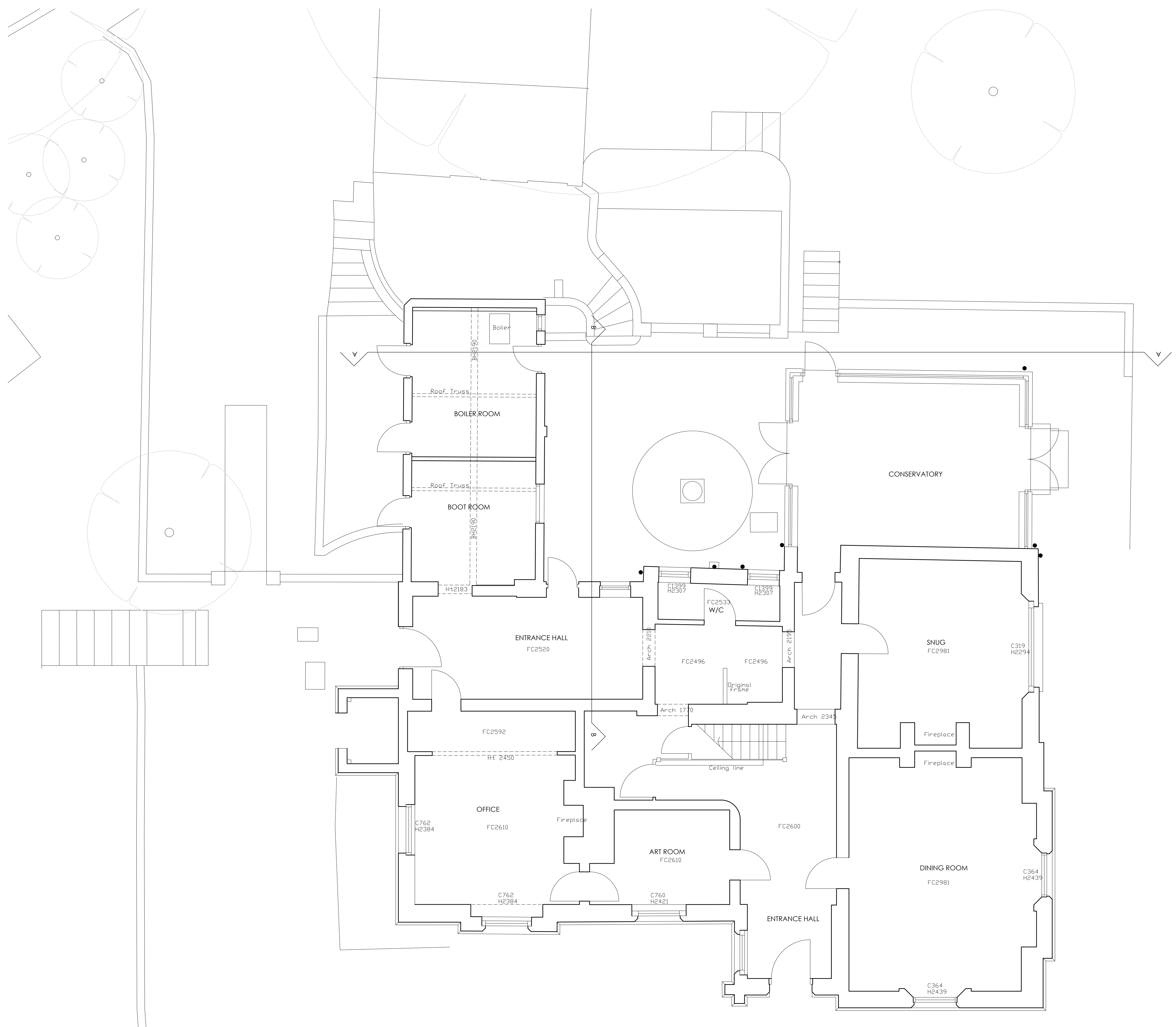
EXISTING GROUND FLOOR PLAN Scale 1/ 50
