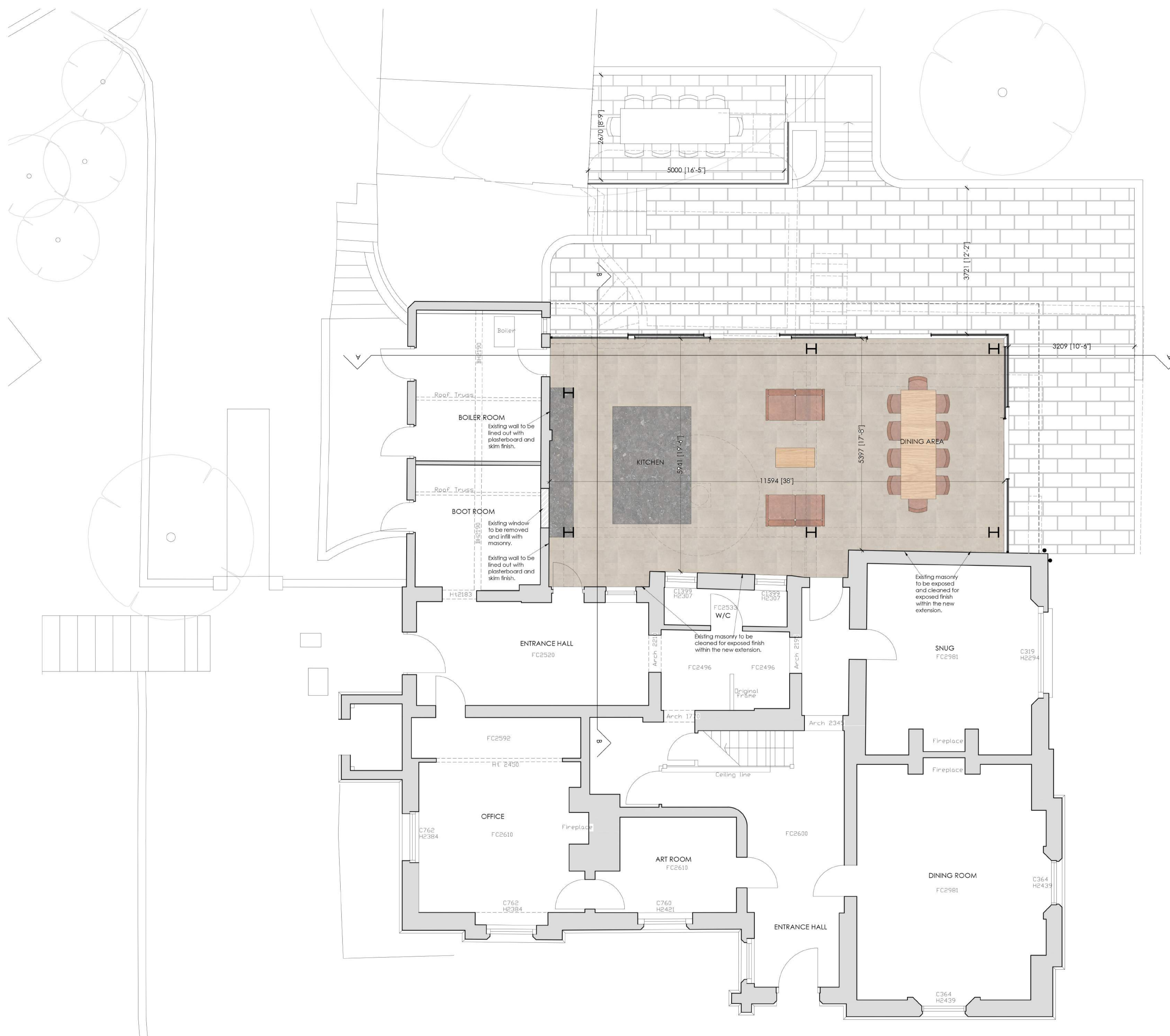
PROPOSED GROUND FLOOR PLAN Scale 1/ 50
