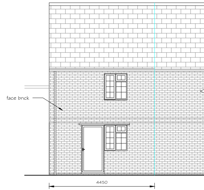
EXISTING SOUTH ELEVATION (REAR)
