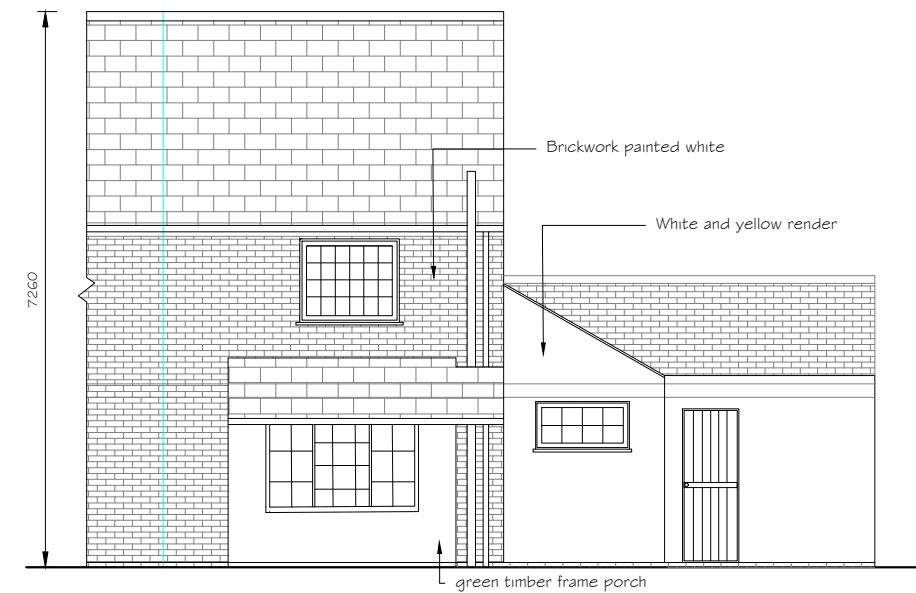
EXISTING NORTH ELEVATION (FRONT)
