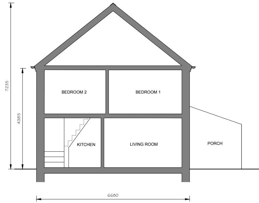
EXISTING EAST SECTION / ELEVATION
