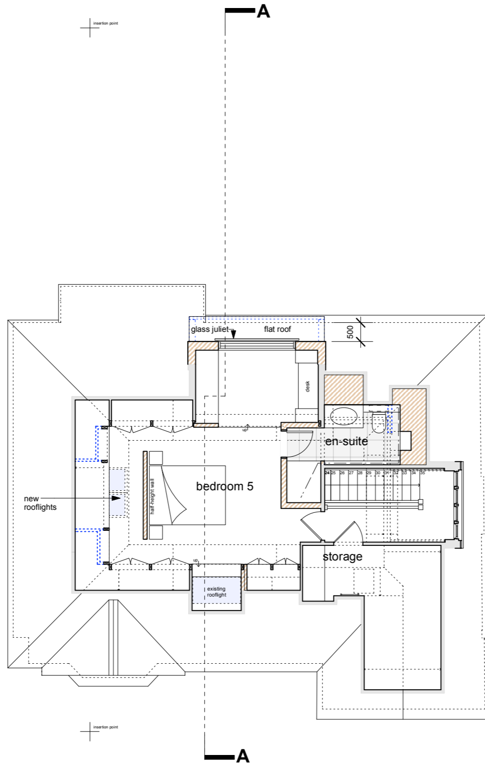
Second Floor Plan Option One
