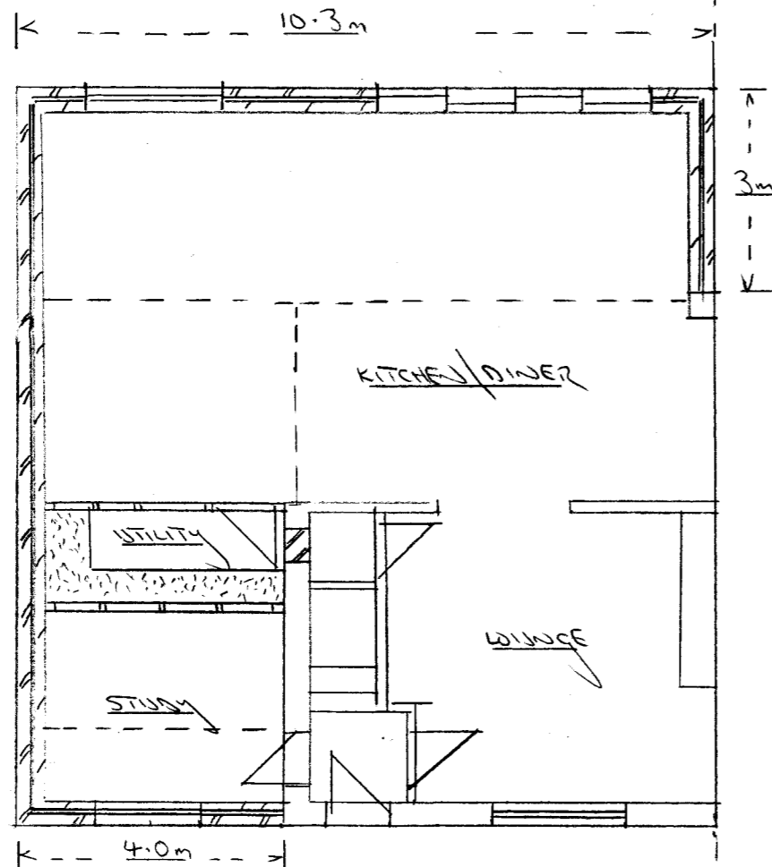
PROP G.F. PLAN
