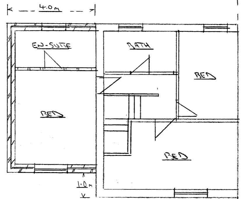
PROP F.F. PLAN
