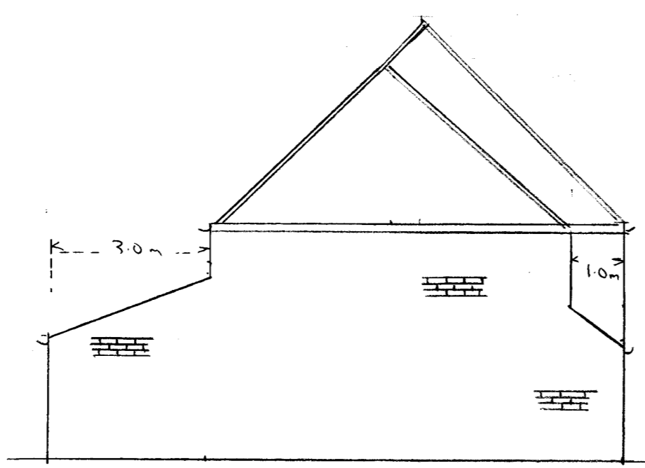
PROP SIDE VIEW
