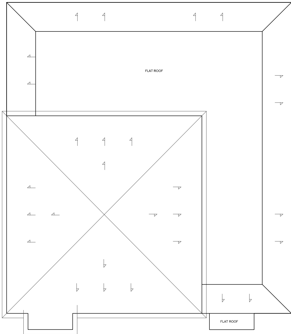
ROOF PLAN
