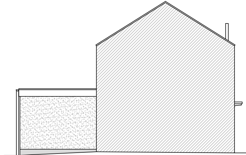
LEFT ELEVATION
