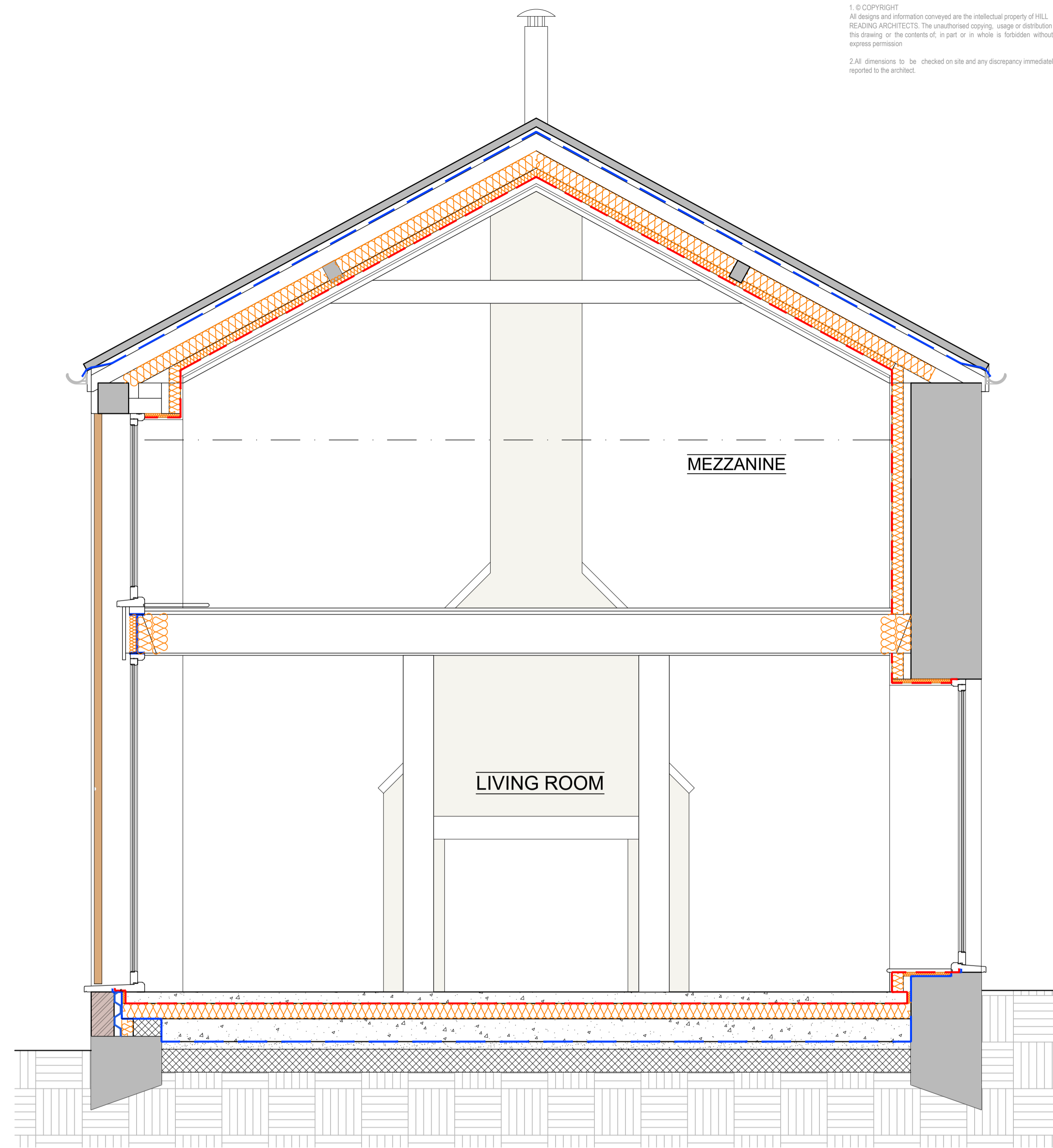
SECTION B-B [SCALE 1:20]
