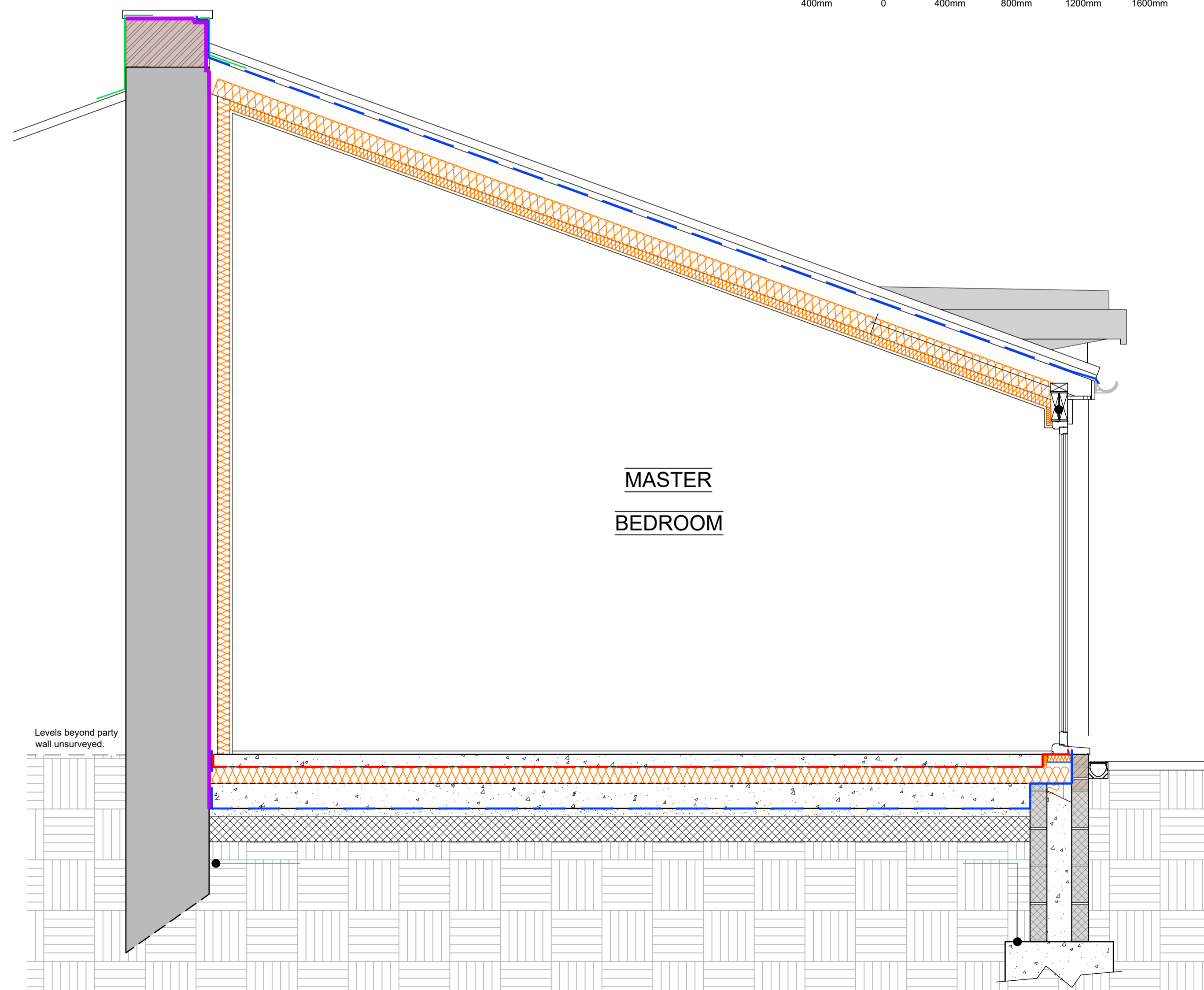
SECTION D-D [SCALE 1:20]
