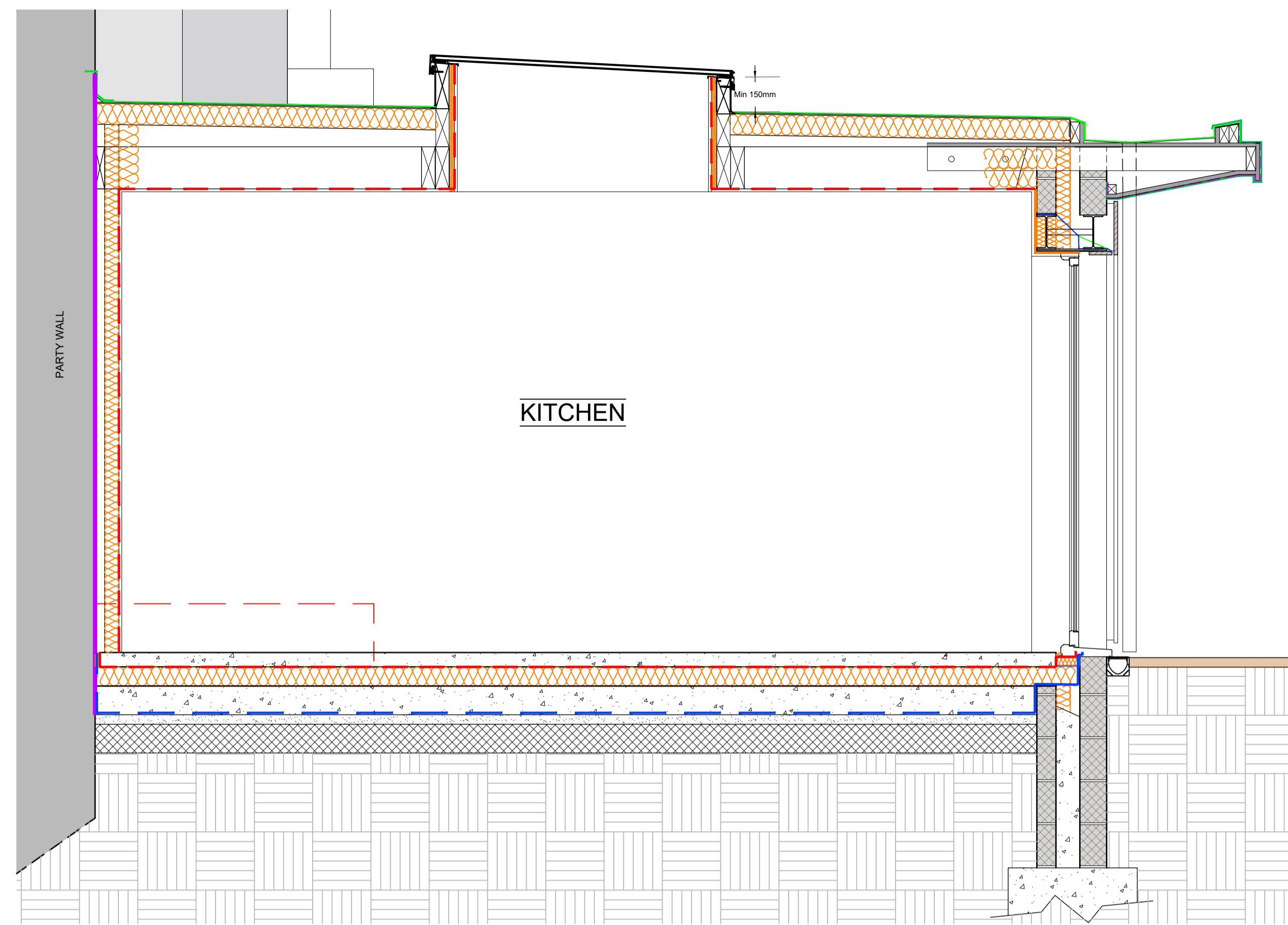
SECTION C-C [SCALE 1:20]
