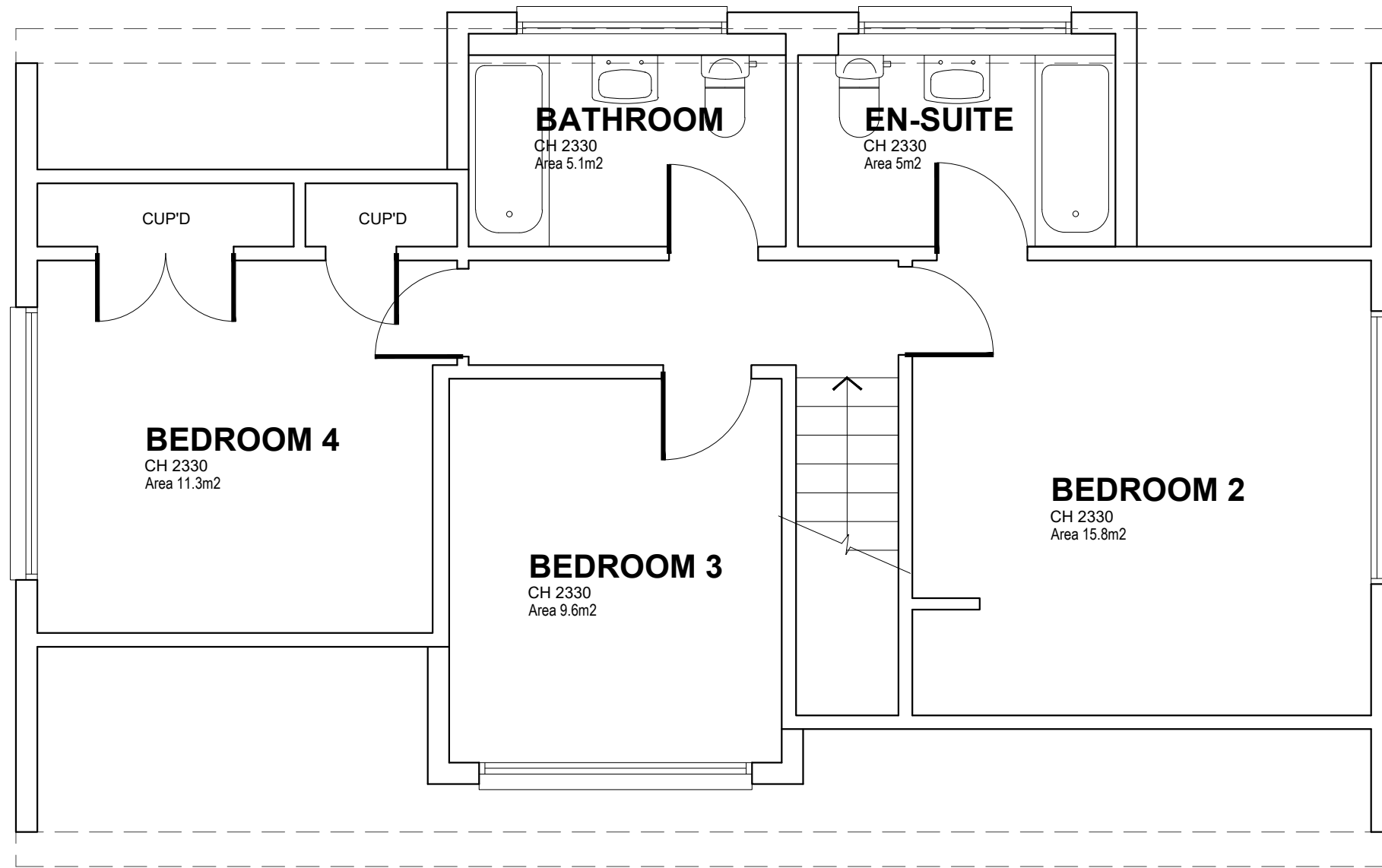
EXISTING FIRST FLOOR LAYOUT SCALE 1:50
