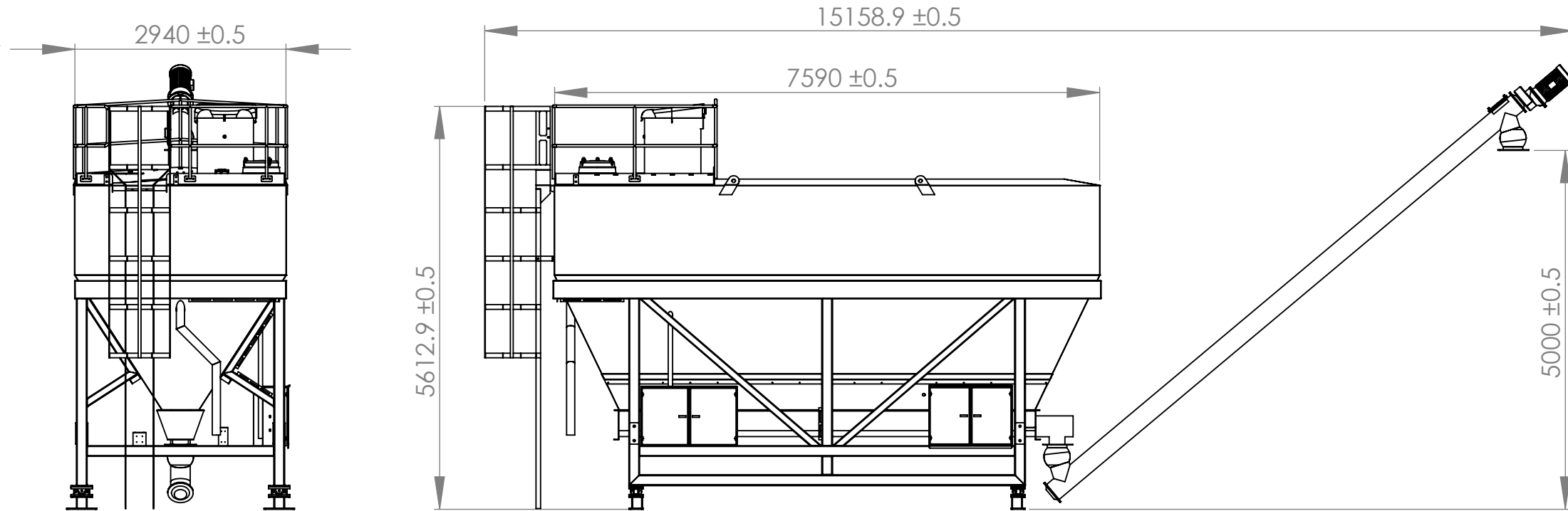
60T Horizontal silo with custom legs and load cells
