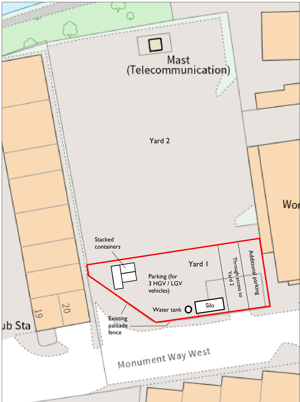
Block Plan (1:500)
