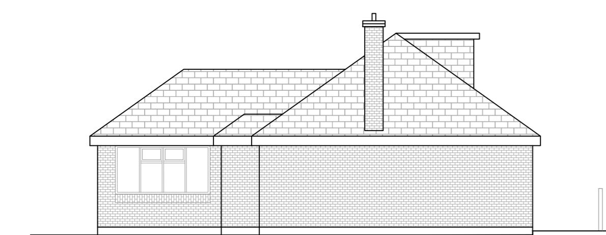
EXISTING RIGHT HAND SIDE ELEVATION 1 : 100
