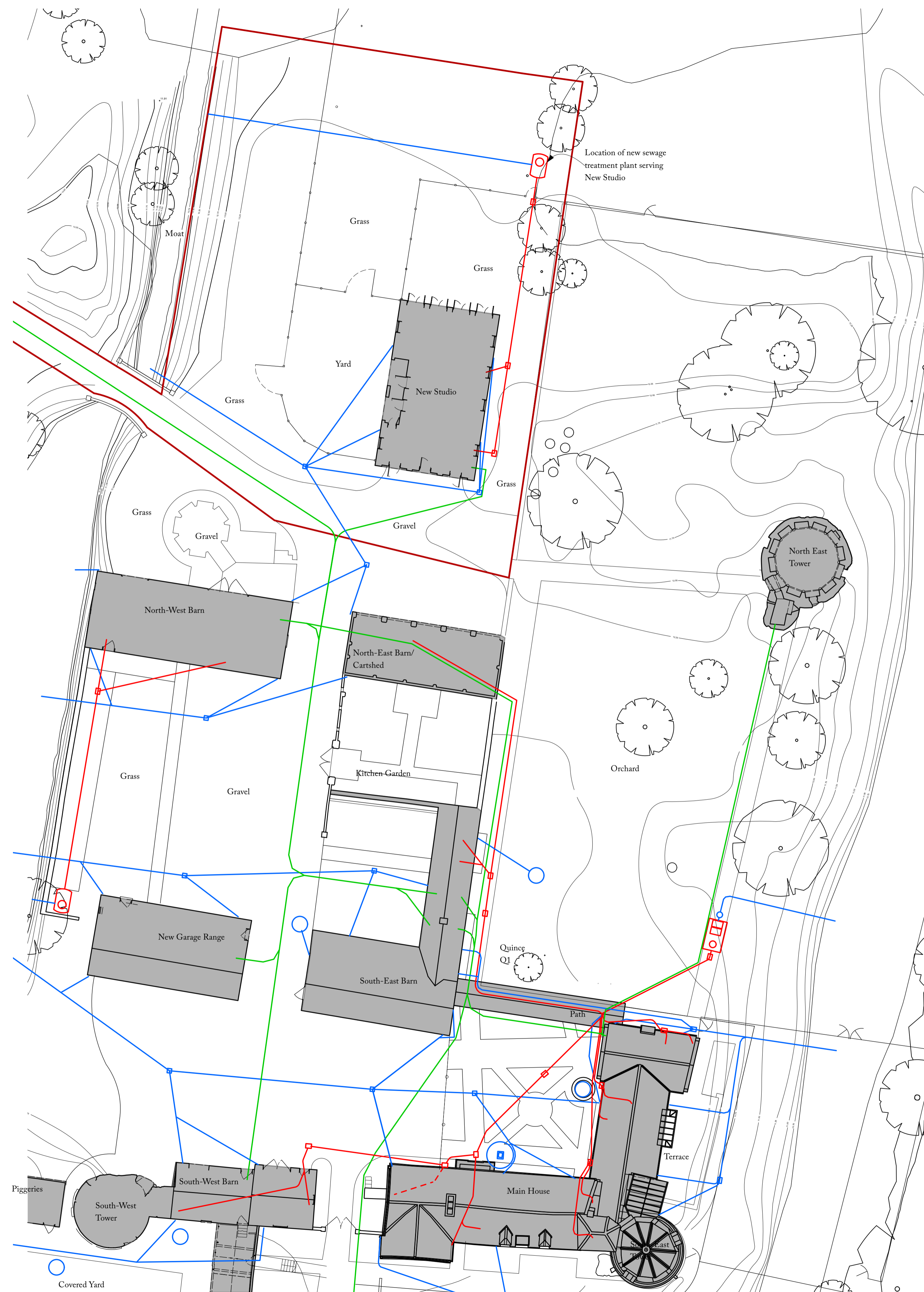
BLOCK PLAN AS PROPOSED 1:250 at A1/ 1:500 at A3
