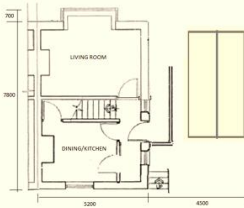
EXISTING GROUND FLOOR MEASUREMENTS
