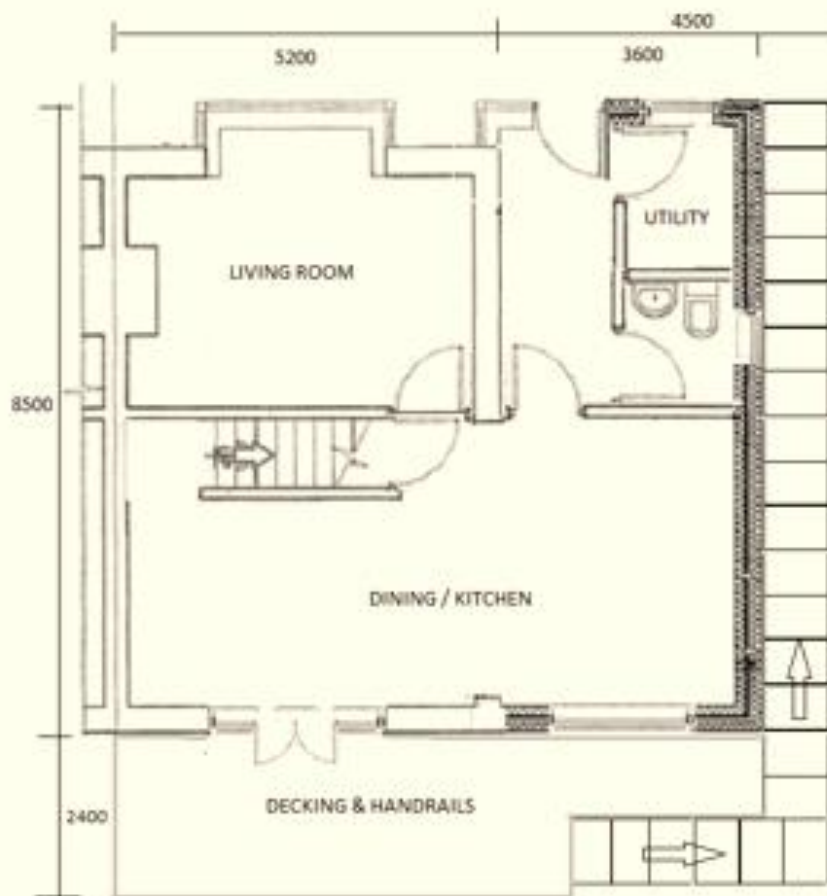
PROPOSED GROUND FLOOR MEASUREMENTS
