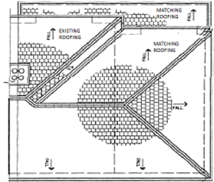
PROPOSED ROOFING PLAN
