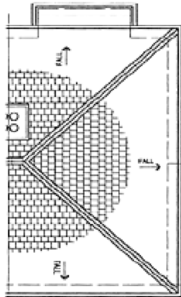
EXISTING ROOFING PLAN
