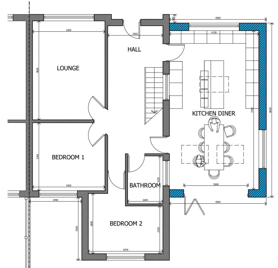
3. Proposed Ground Floor Layout
