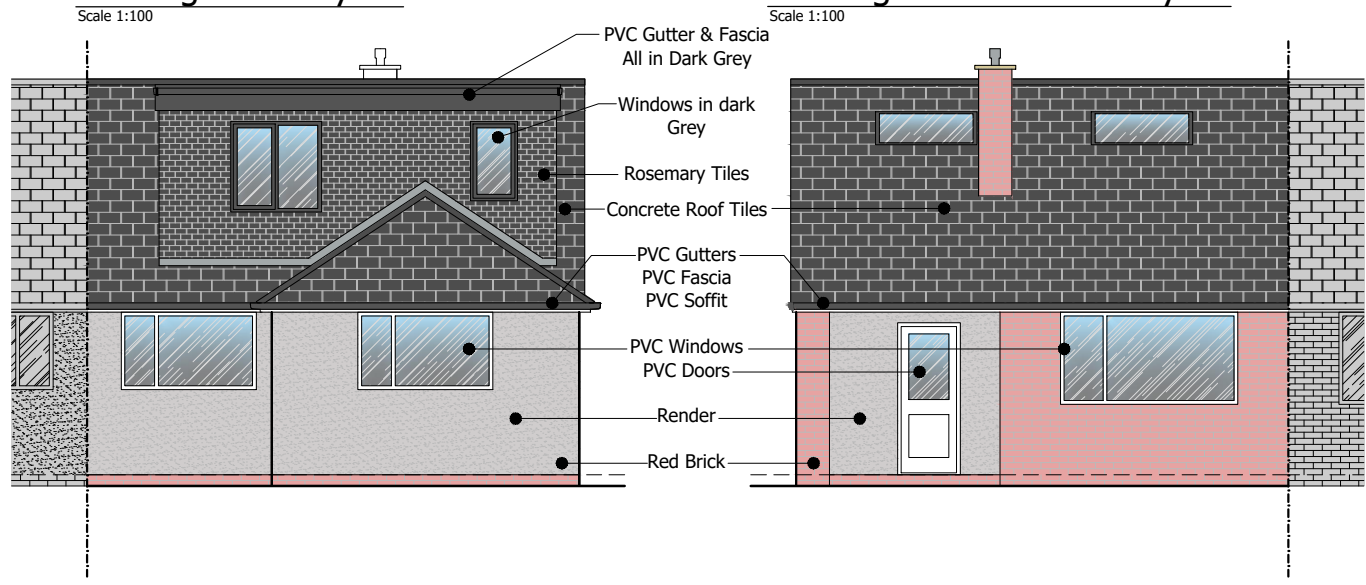
5. Existing East Elevation
