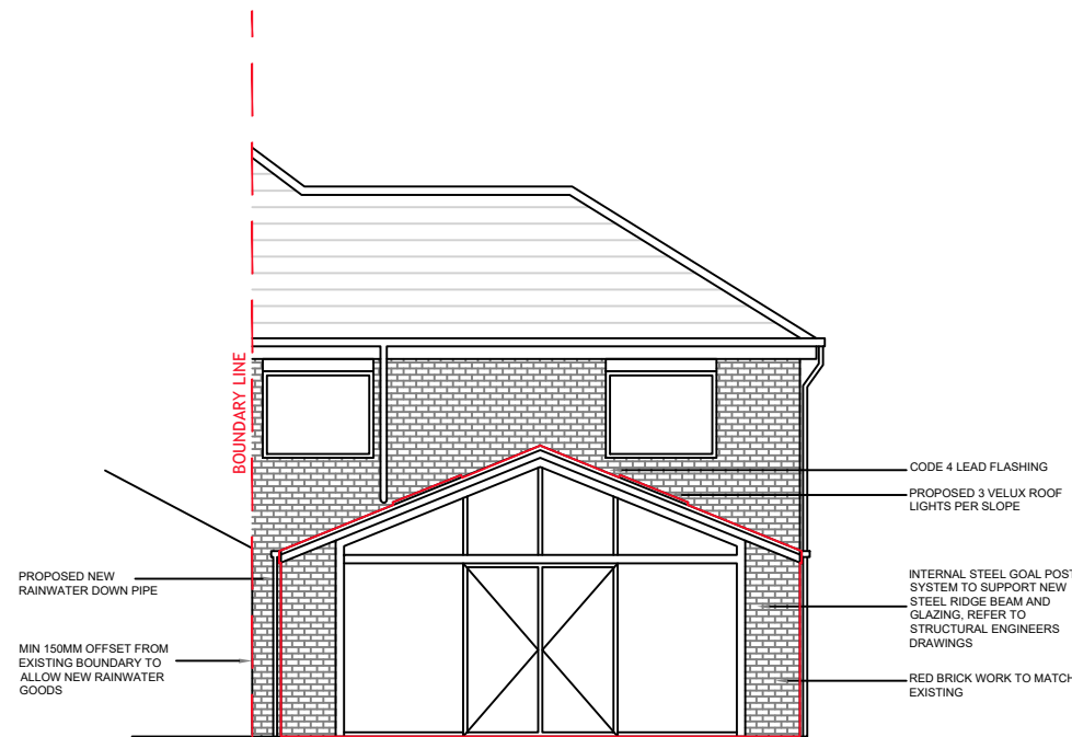
Proposed Rear Elevation 1:100 @A3
