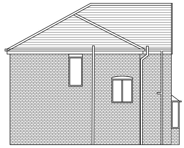
Existing Side Elevation 1:100 @A3
