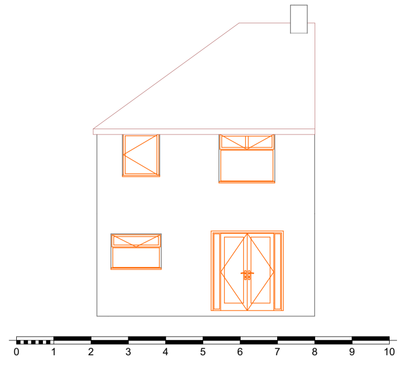
1 East Elevation Existing 1:100
