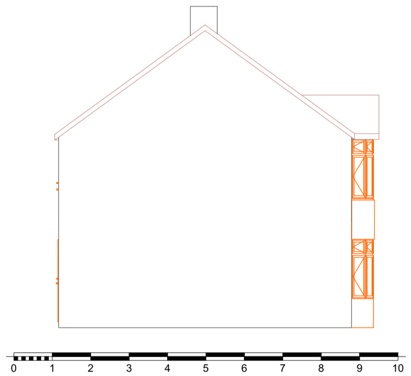
3 North Elevation Existing 1:100
