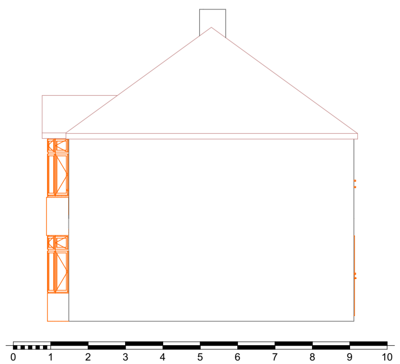
4 South Elevation Existing 1:100
