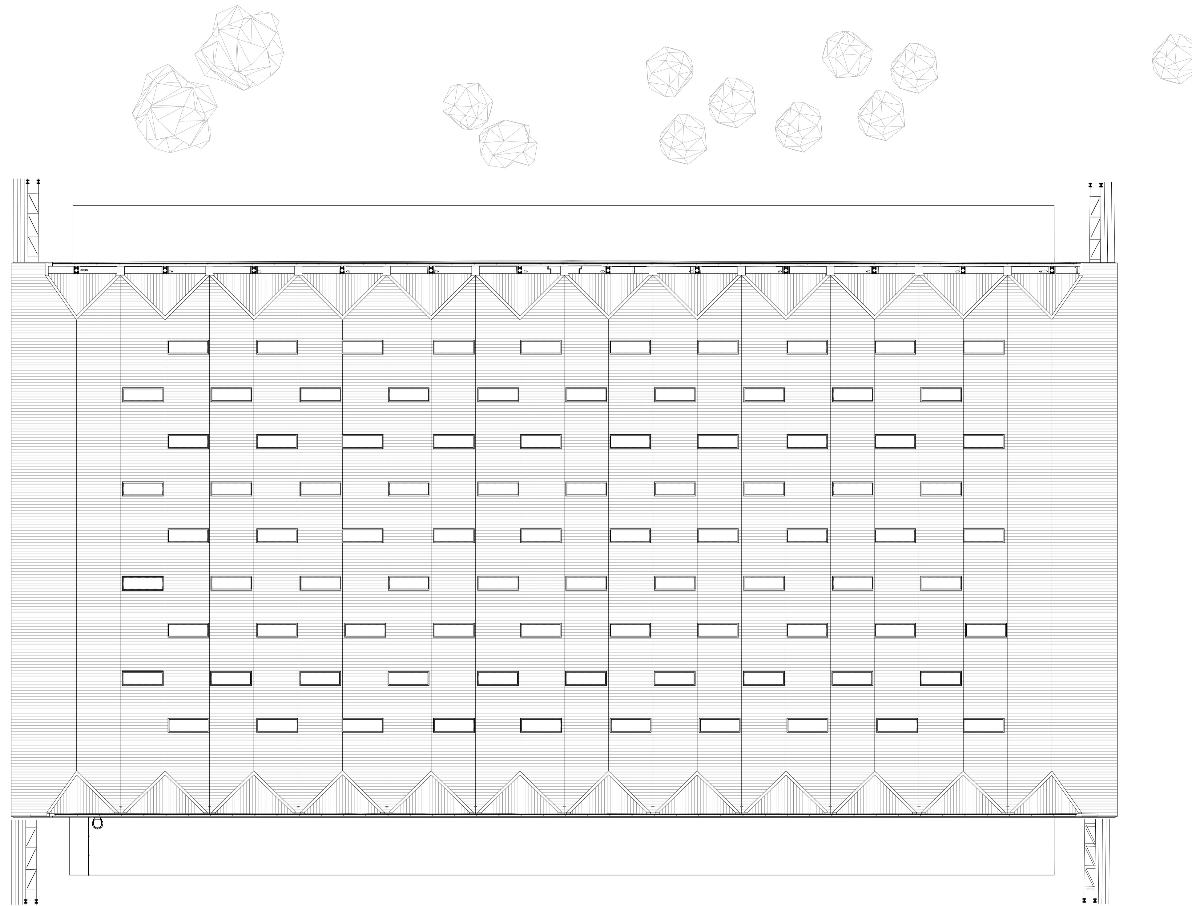
1. Existing Roof Plan SCALE - 1 : 200@A1
