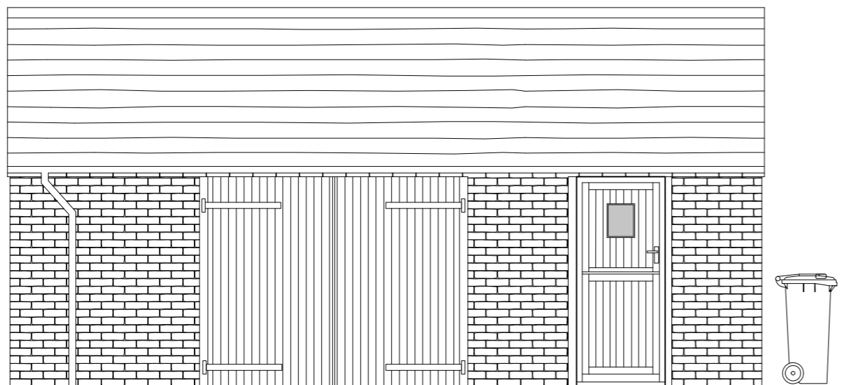
Front Elevation - East
