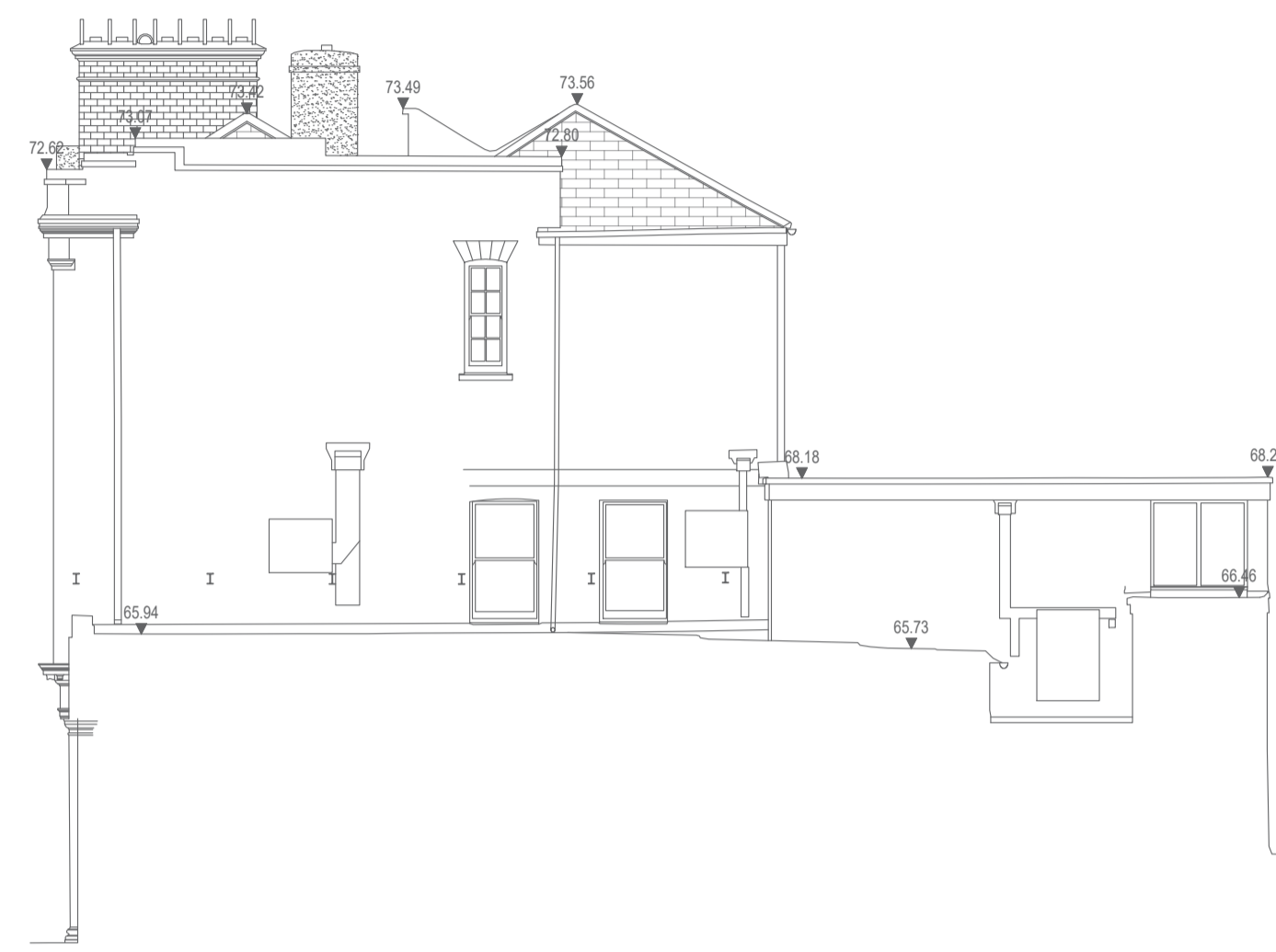
Existing North West (Side) Elevation
