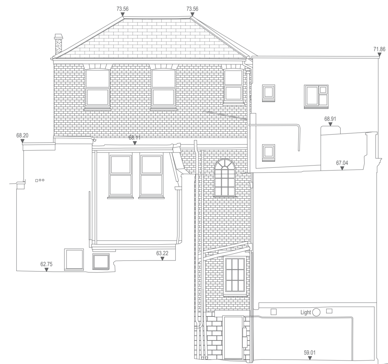
Proposed South West (Rear) Elevation
