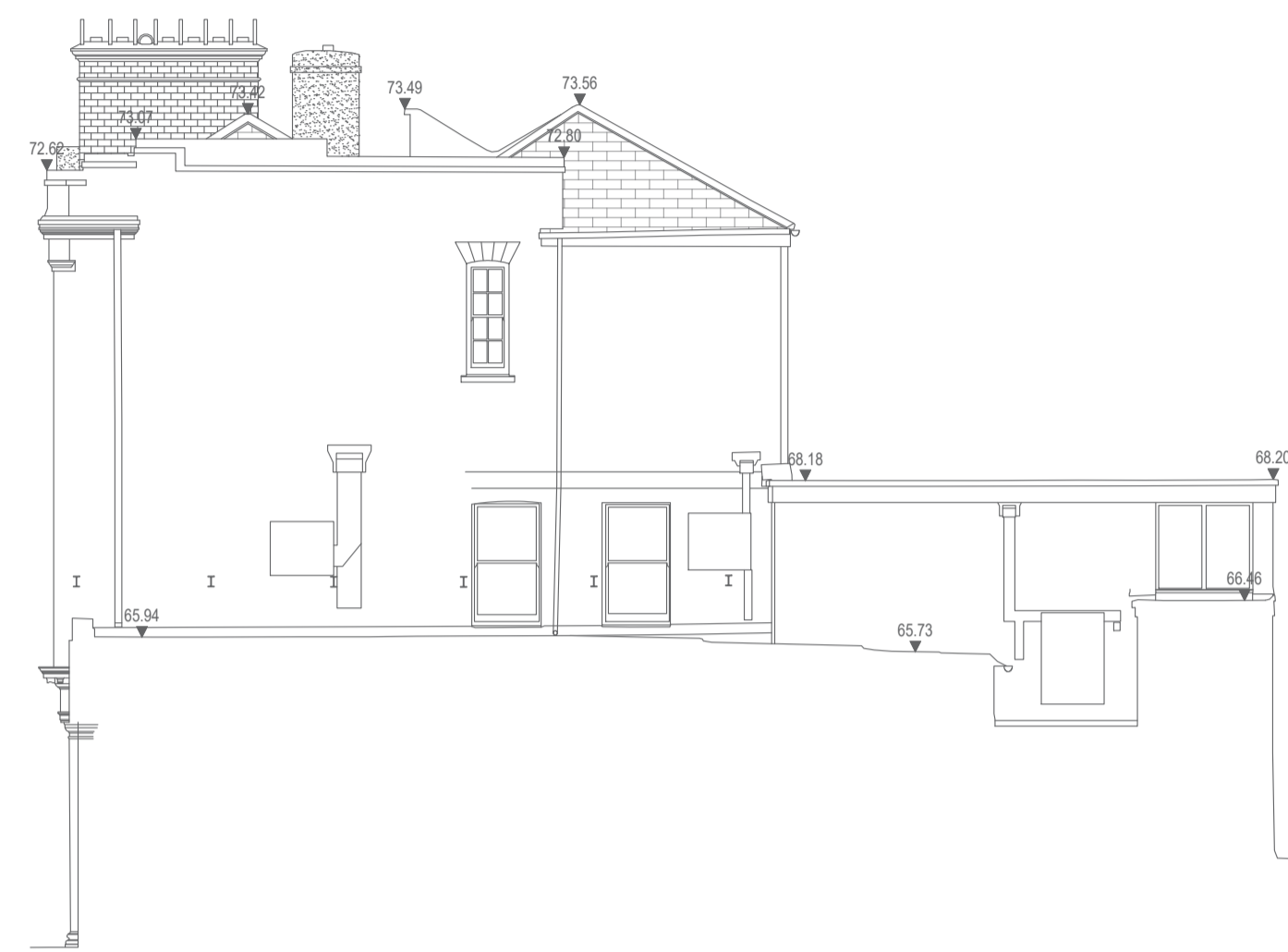
Proposed North West (Side) Elevation
