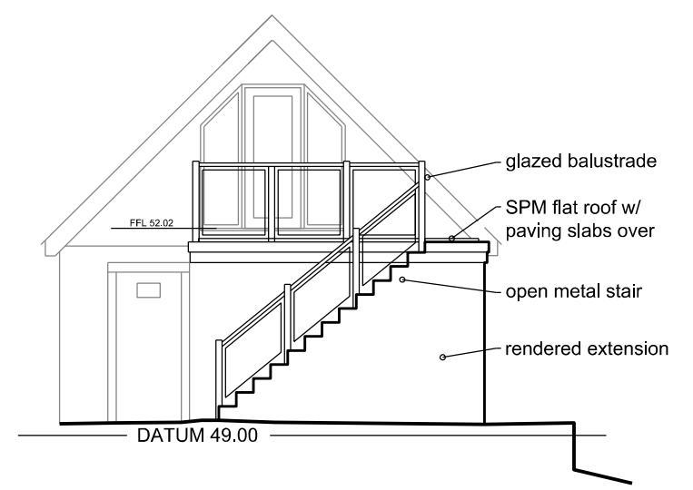
EAST ELEVATION (REAR)
