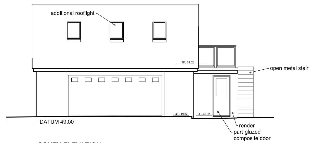
SOUTH ELEVATION
