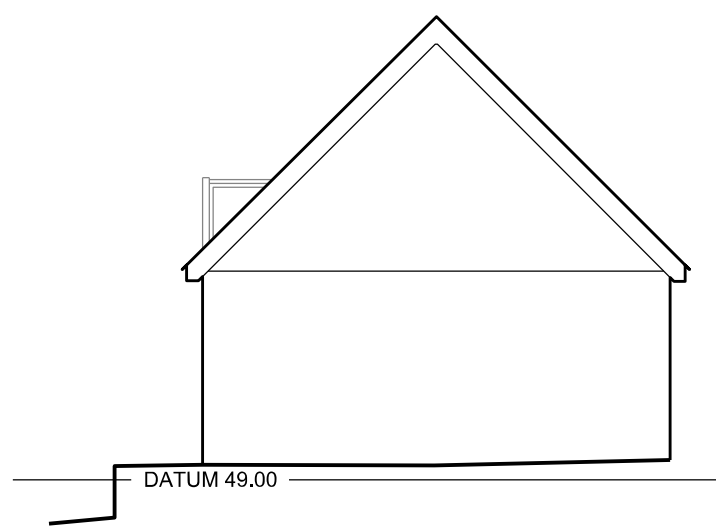
WEST ELEVATION (STREET)
