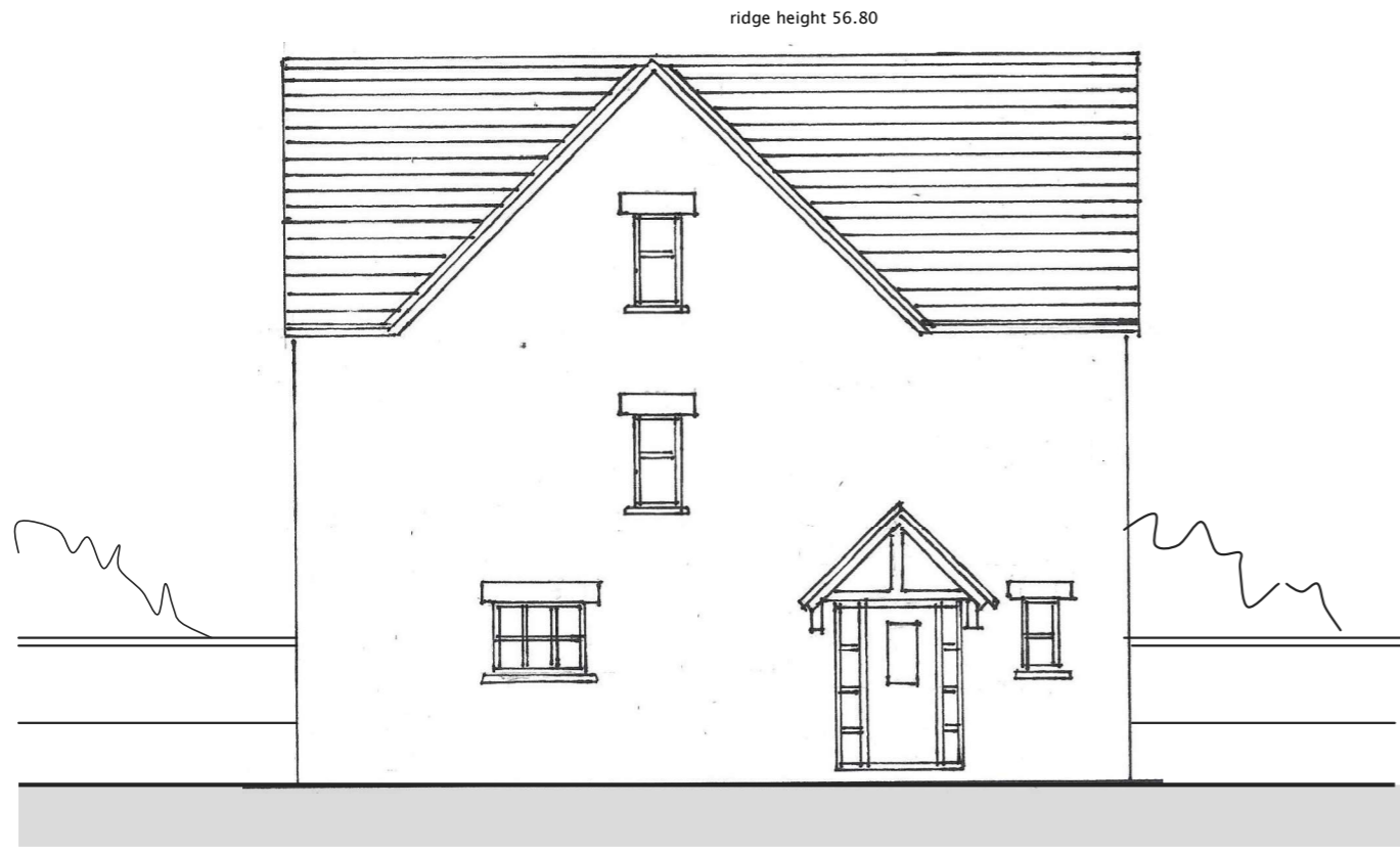
WEST ELEVATION
