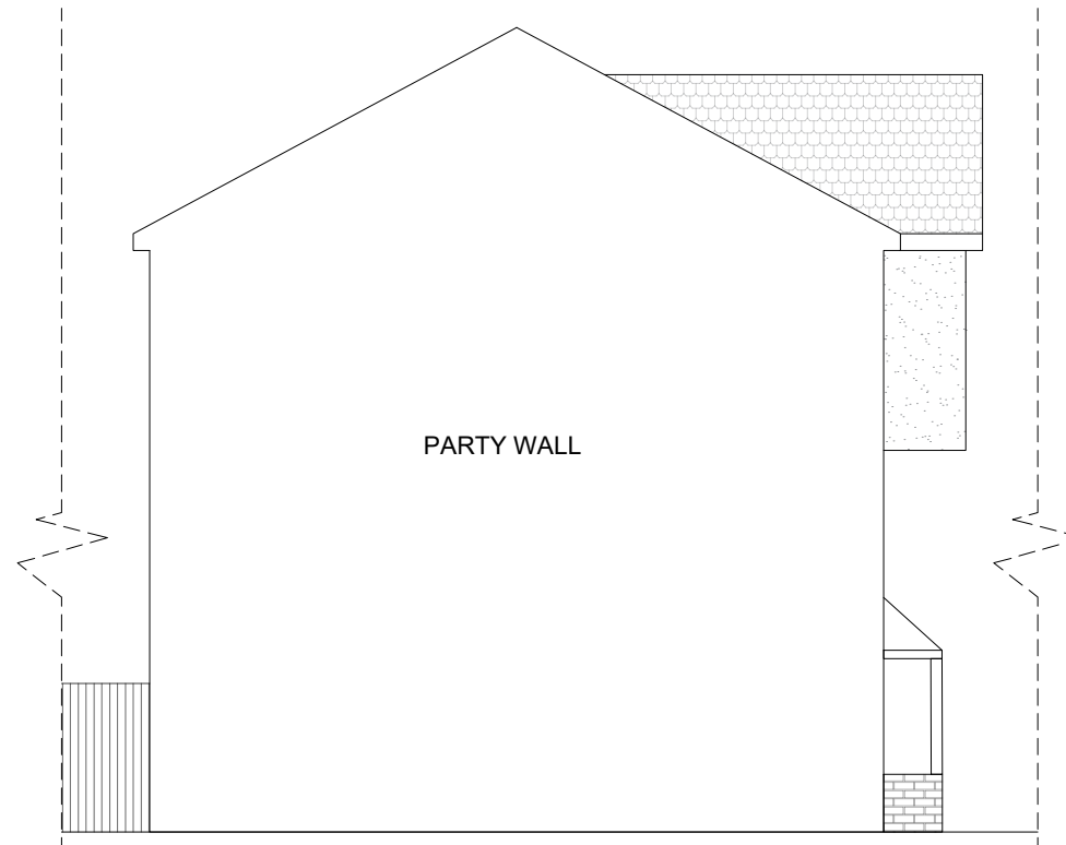
Proposed South Elevation ( No Proposed Change )
