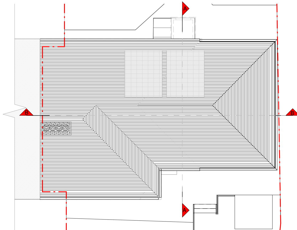
Roof Plan
