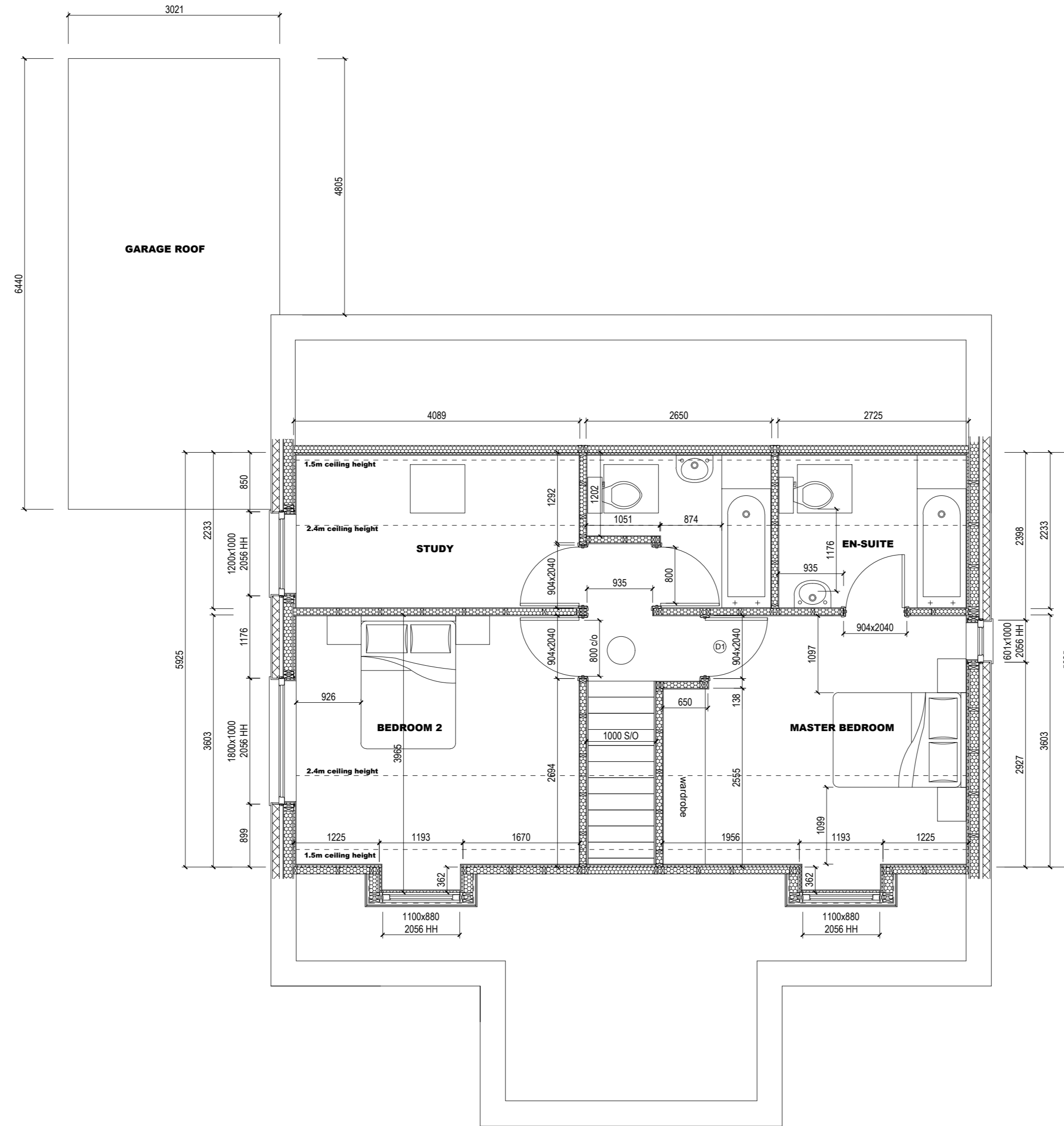
Proposed First Floor Plan 54.608m 2
