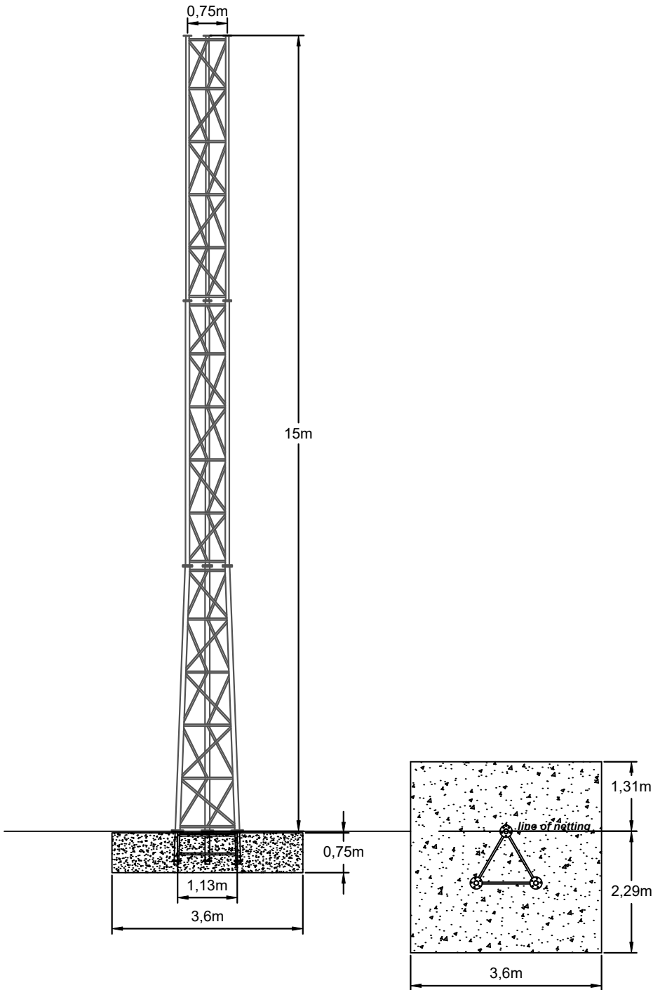
15m golf ballstop netting support tower showing foundation details
