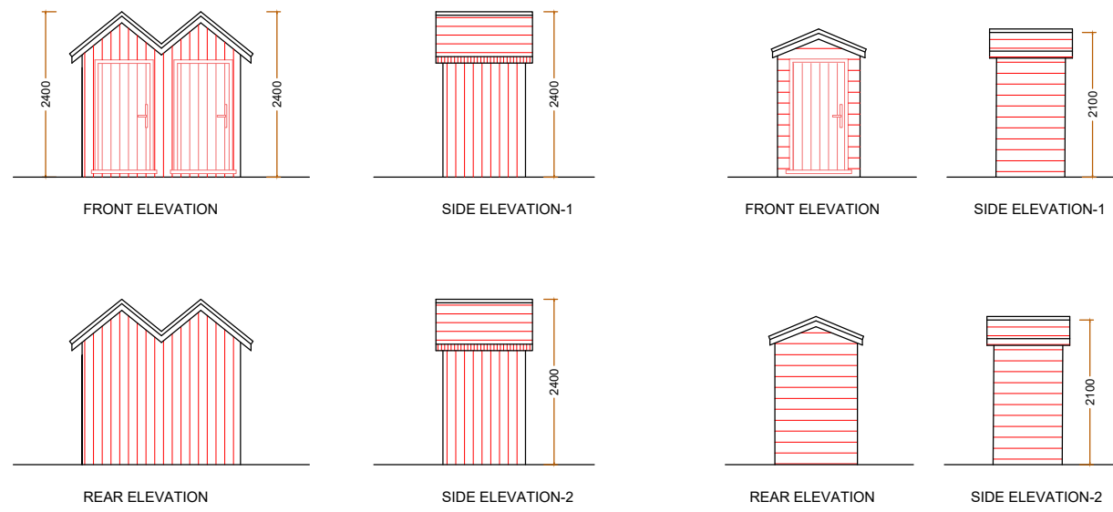
SHED-1
