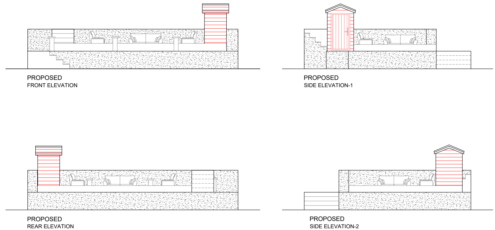
PROPOSED SUNKEN SEATING AREA
