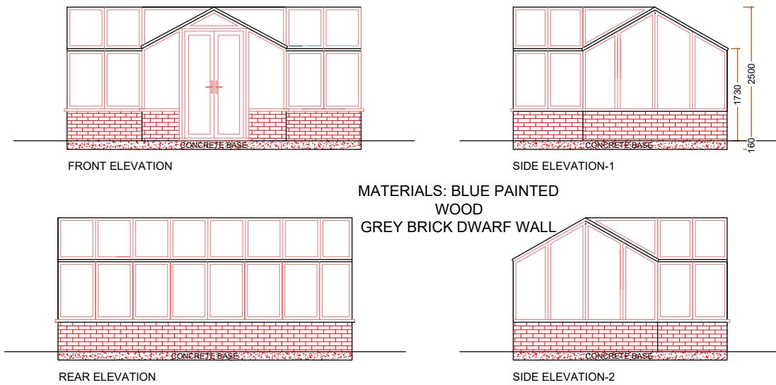
PROPOSED GREENHOUSE
