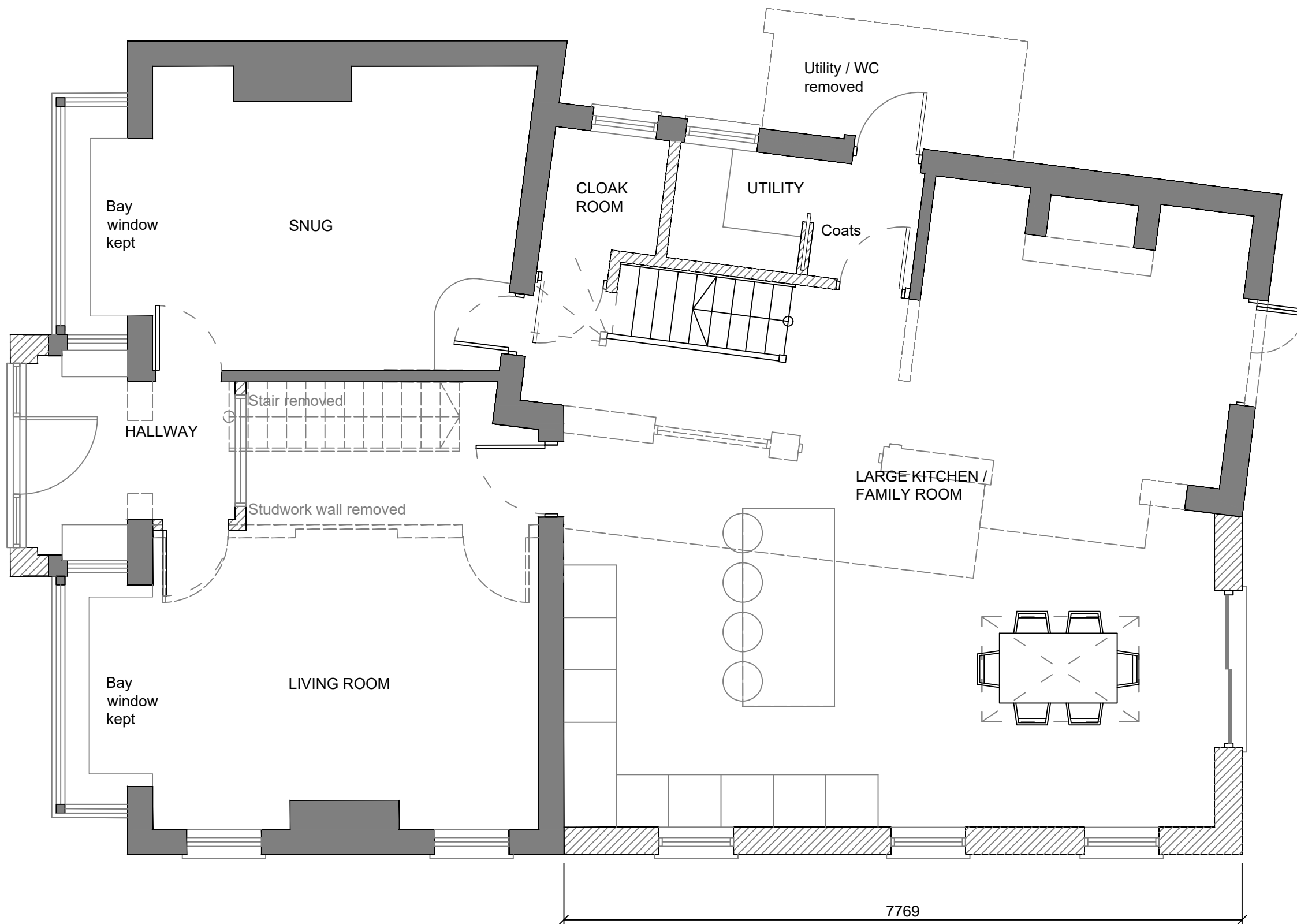
PROPOSED GROUND FLOOR PLAN PRIOR NOTIFICATION APPLICATION
