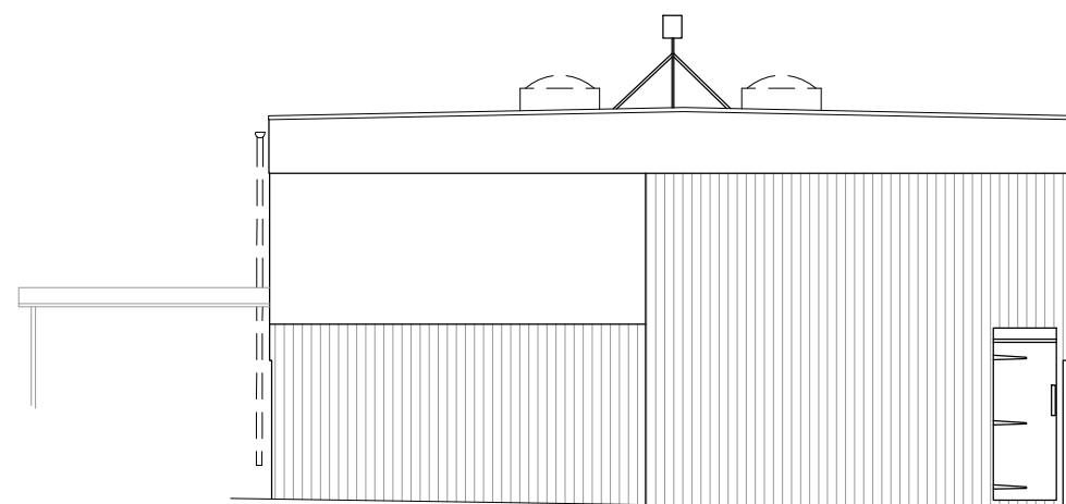
North East Elevation as Existing 1:100
