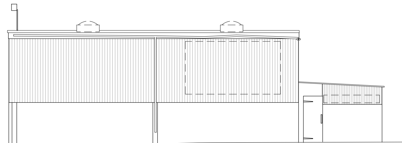
North West Elevation as Existing 1:100
