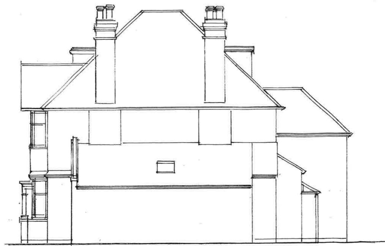
SIDE (WEST) ELEVATION
