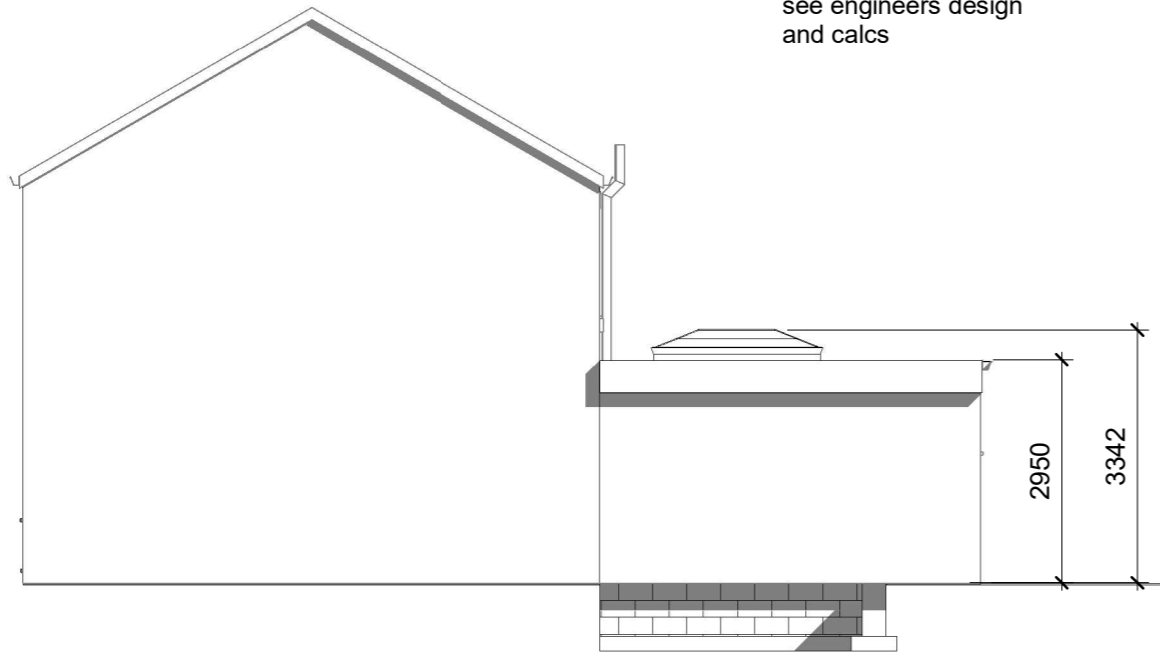
3 Neighbouring Elevation 1 : 100
