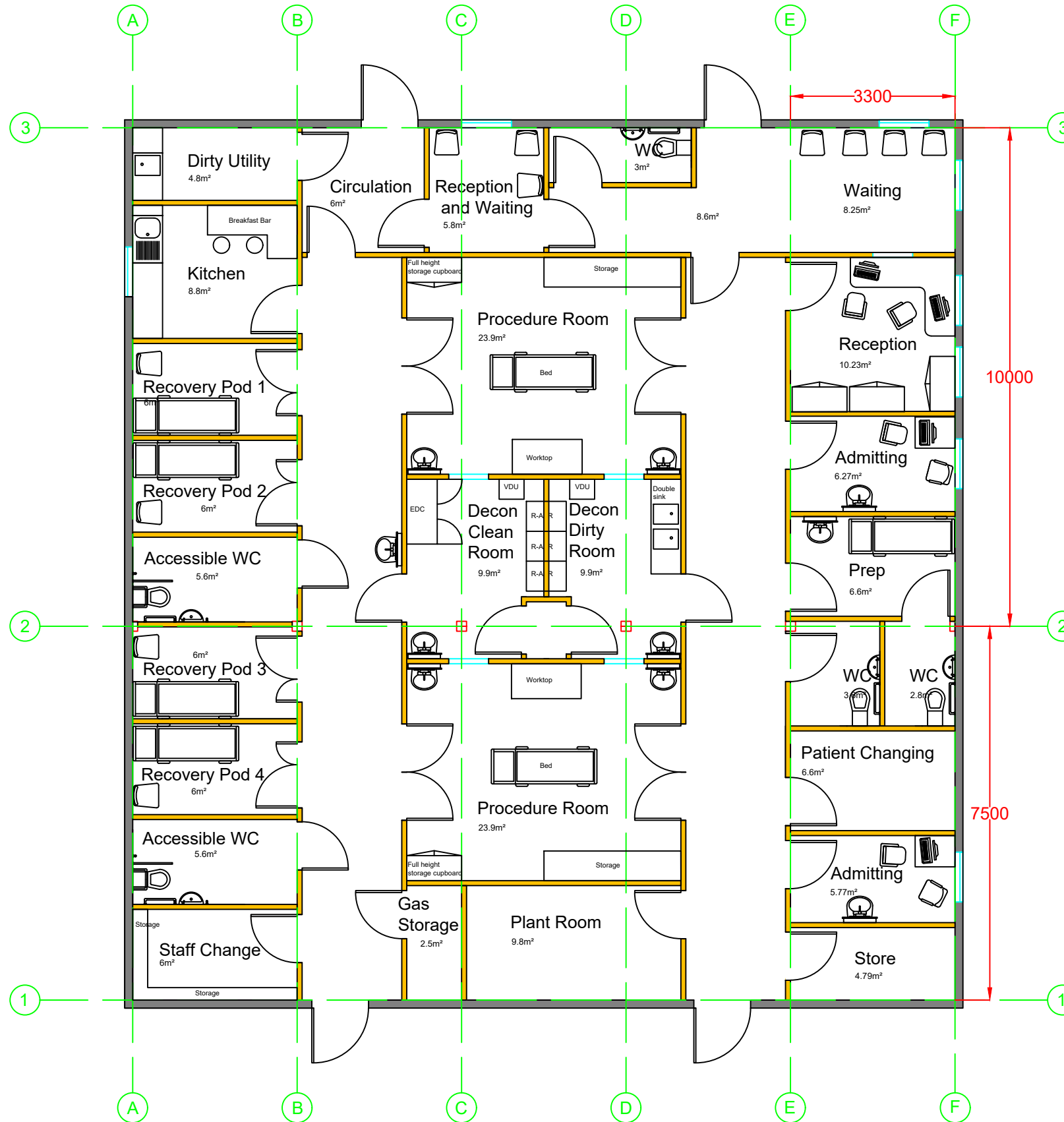
PLAN VIEW - 1:100 @ A3
