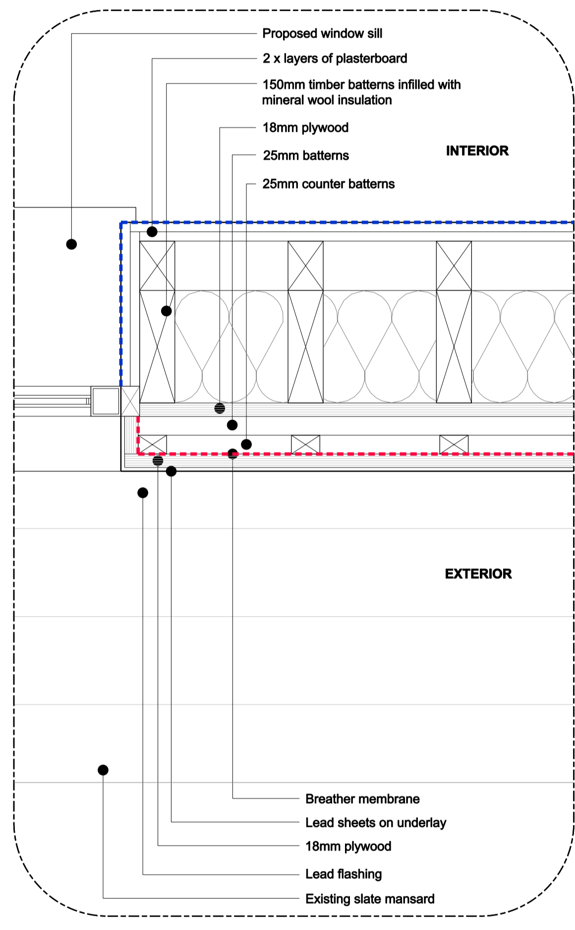
01. Plan Showing Junction of Window and Wall
