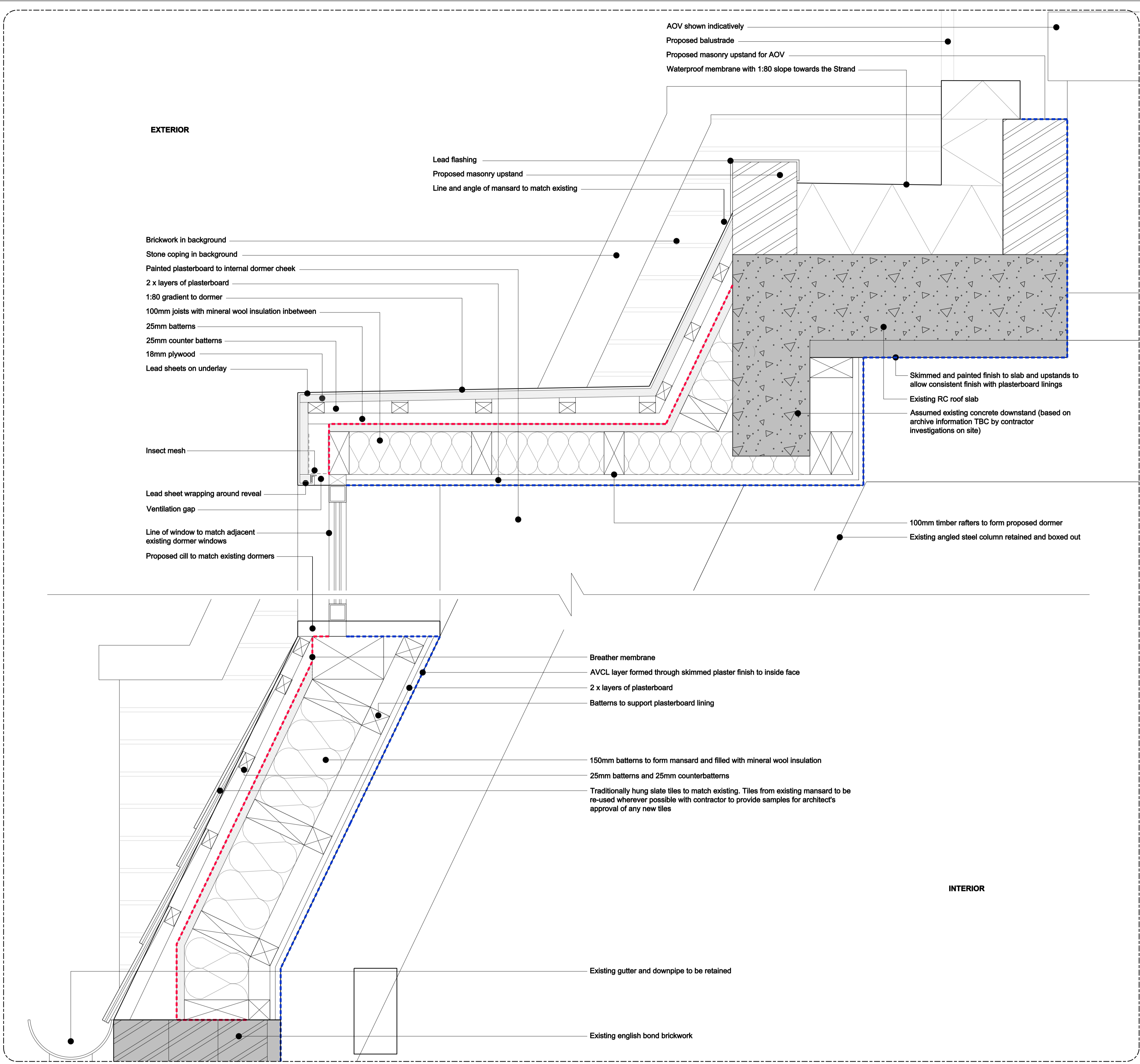
02. Section Through Dormer Window
