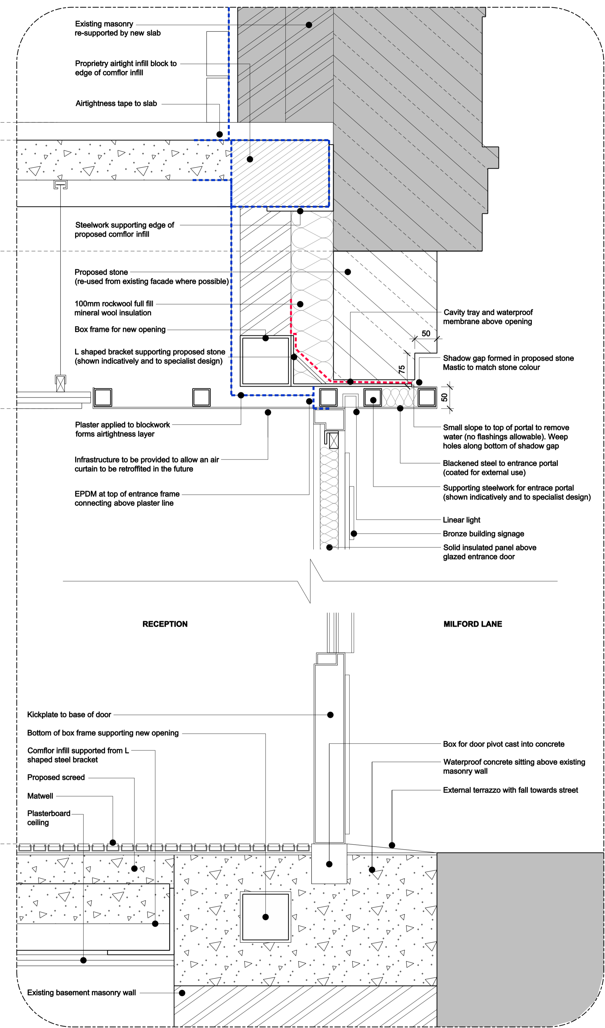
02. Section Showing Top of Metal Entrance Portal and Door
