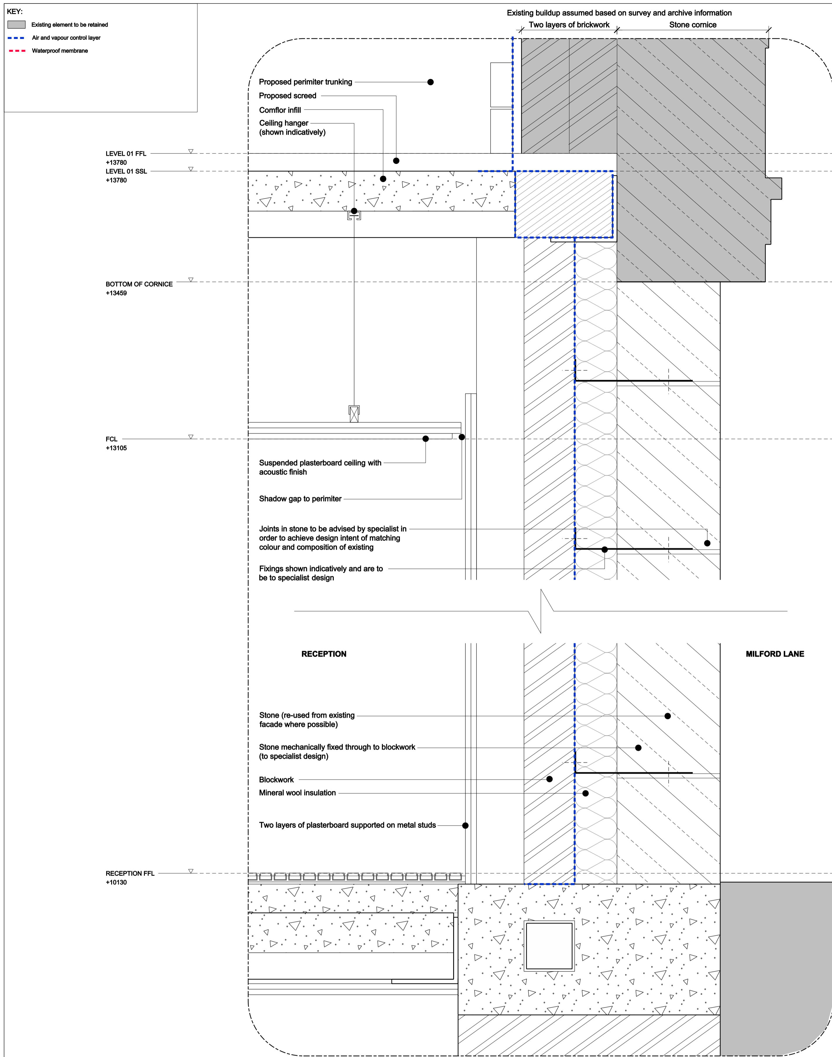
01. Section Showing Build Up of Stone Infills
