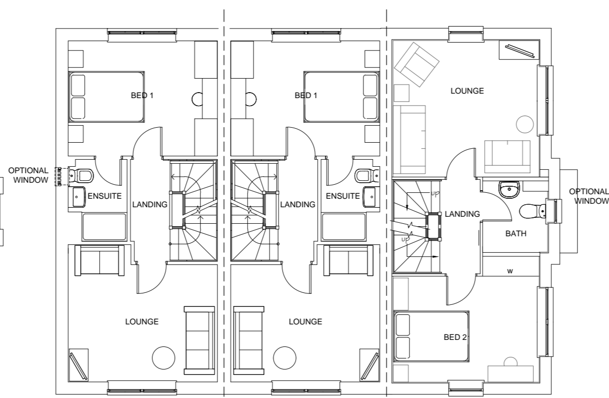
FIRST FLOOR PLAN KINGSVILLE KINGSVILLE BRENTFORD
