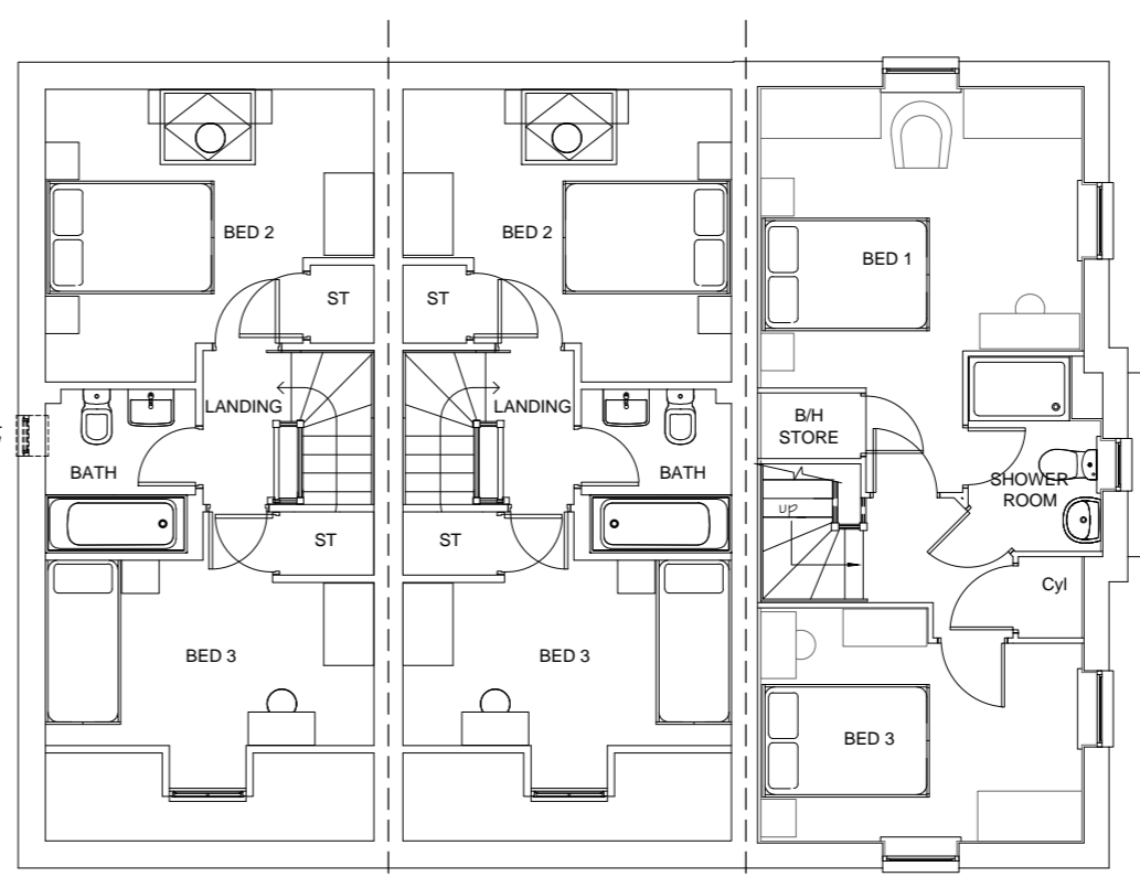
SECOND FLOOR PLAN KINGSVILLE KINGSVILLE BRENTFORD
