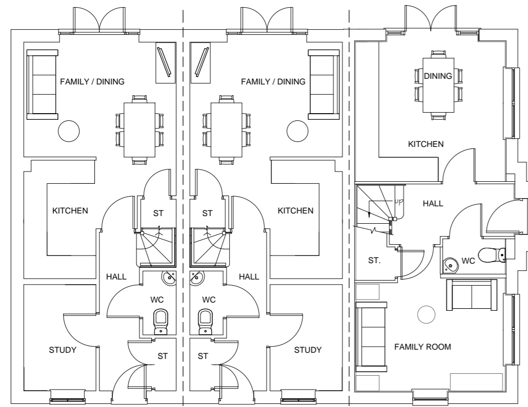
GROUND FLOOR PLAN KINGSVILLE KINGSVILLE BRENTFORD
