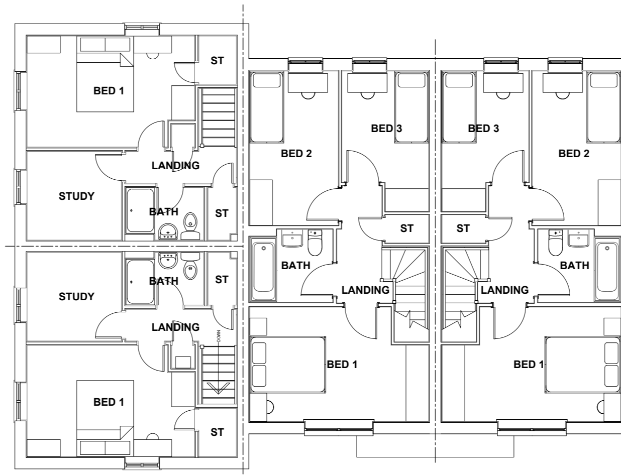
FIRST FLOOR PLAN AMBERS
