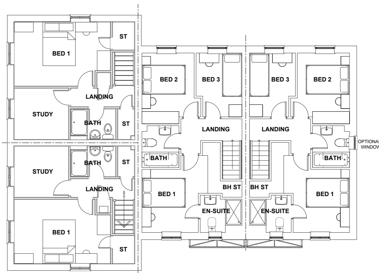
FIRST FLOOR PLAN AMBERS
