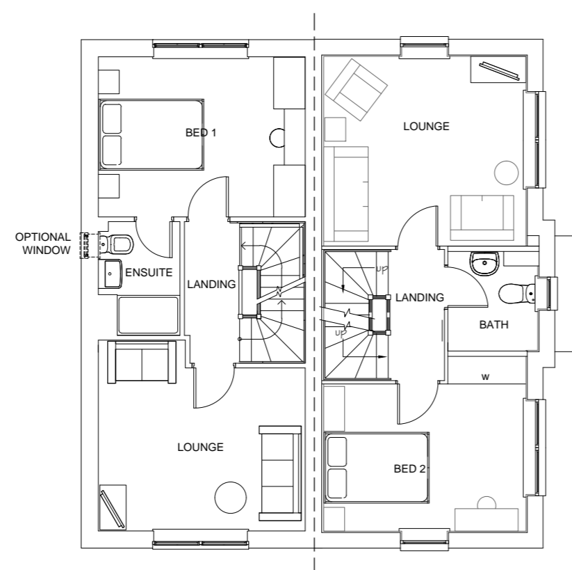
FIRST FLOOR PLAN KINGSVILLE BRENTFORD
