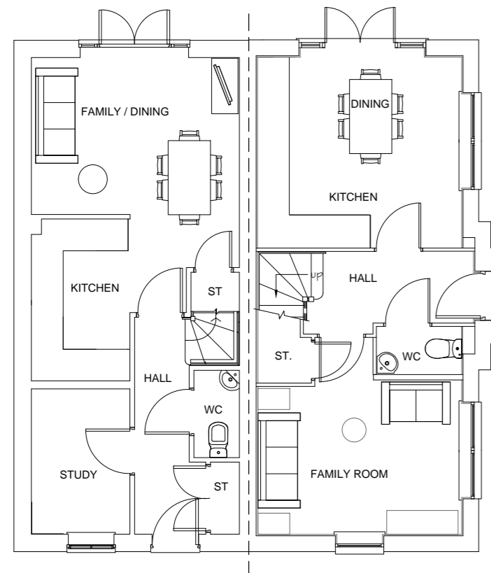
GROUND FLOOR PLAN KINGSVILLE BRENTFORD
