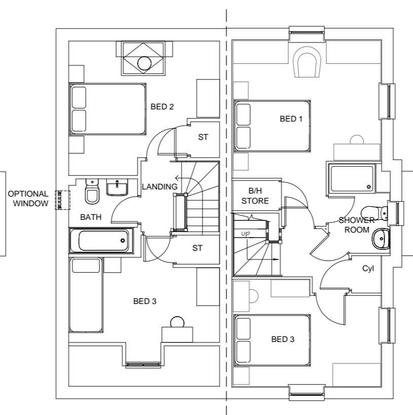
SECOND FLOOR PLAN KINGSVILLE BRENTFORD
