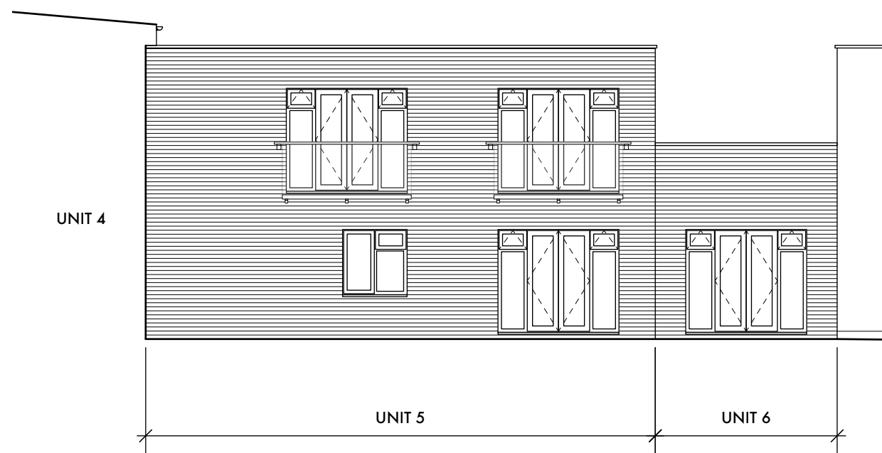
SOUTH-EAST ELEVATION
