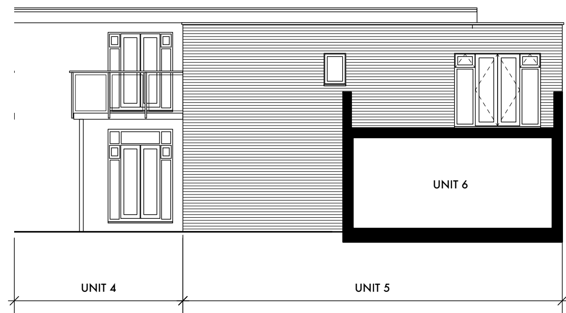
NORTH-EAST ELEVATION
