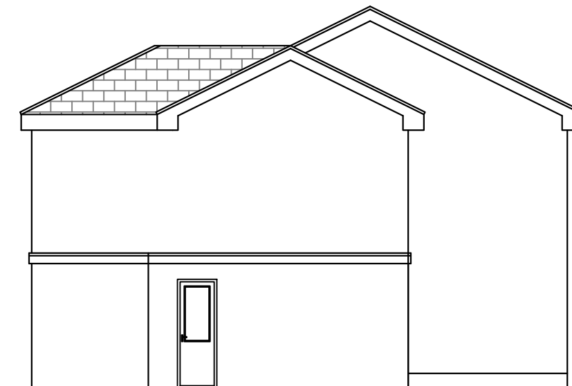
Side Elevation
