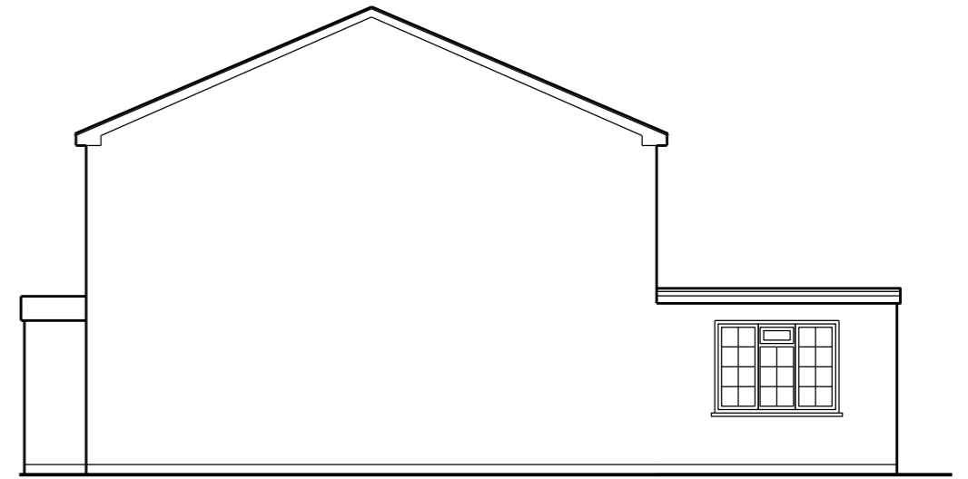
Proposed South East Elevation
