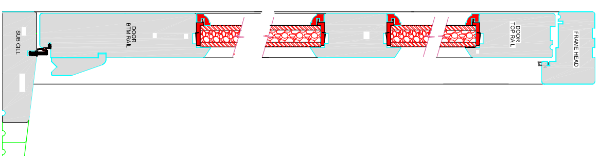
SECTION BB scale 1/5 @ A3
